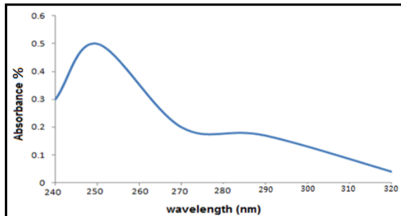
Fig3. UV absorption spectra of ZnO nano particles.
