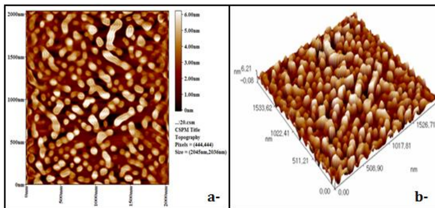
Fig 4:AFM images of ZnO nano prticles, a- in two dimation ,b- in three dimation.
