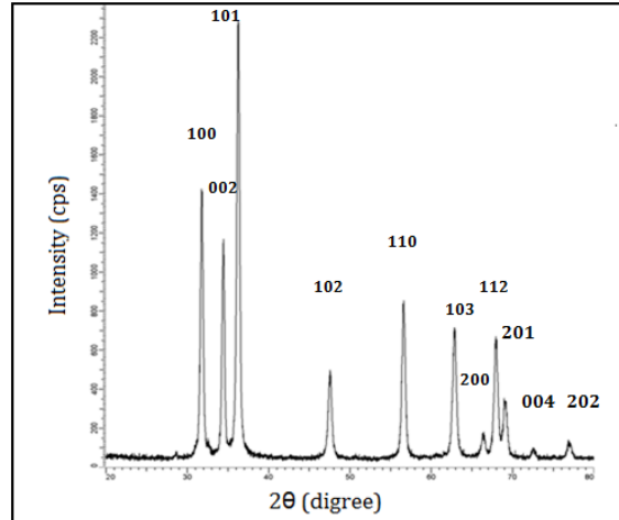
Fig 1: shows X-ray diffraction of ZnO nano particles .
