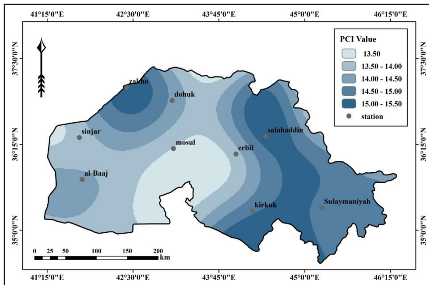
Map 5 Rainfall Concentration Index (PCI1) for autumn
