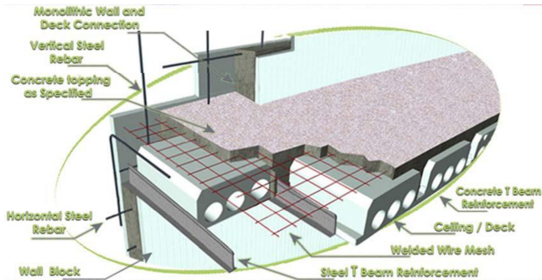
Figure (1) slab element
