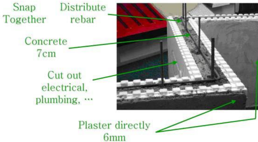
Figure (2)the main structural wall elements
