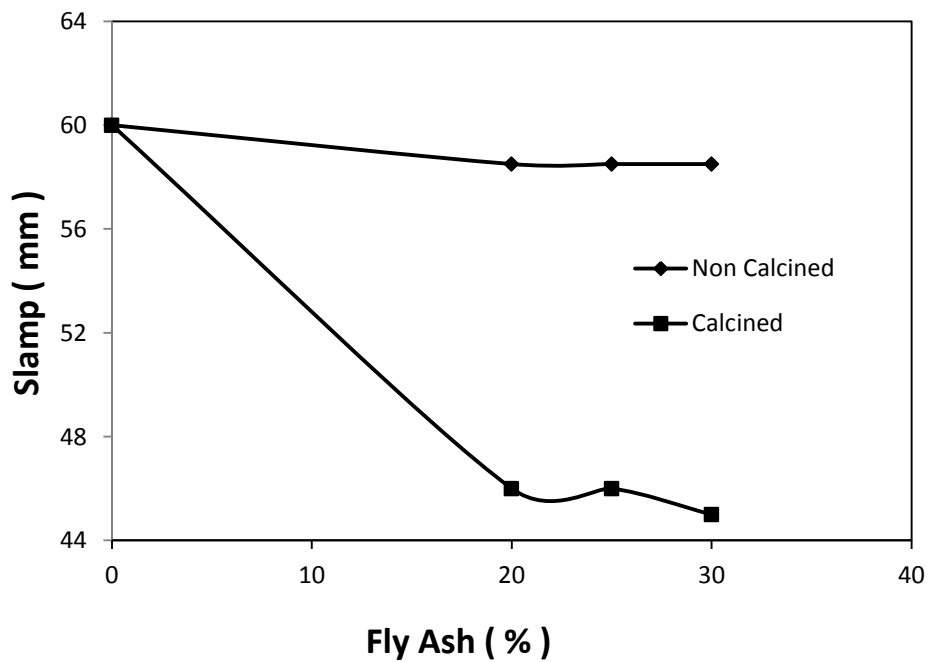
Fig.(4): The Slump of fresh concrete after adding the calcined
