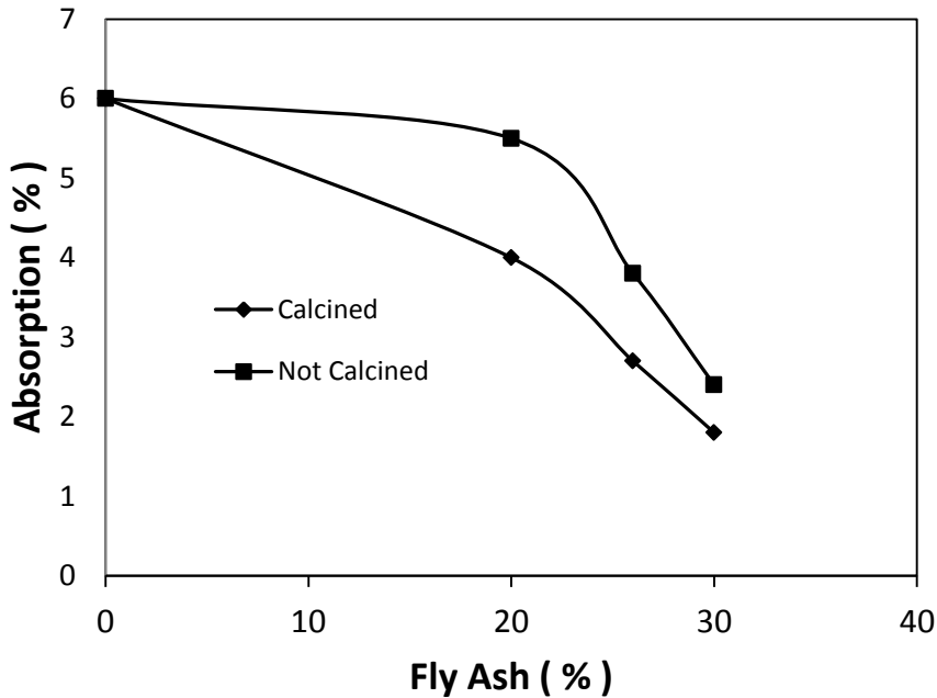
Fig.(5) Absorption ability of the concrete with addition of calcined and non calcined fly ash
