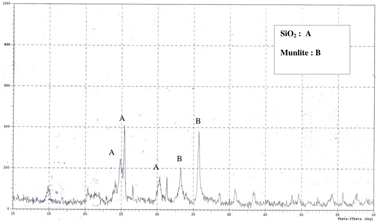
Fig.(3): X-Ray pattern of calcined fly ash
