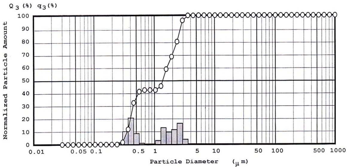
Fig.(2): particle size analysis for Calcined Fly Ash.
