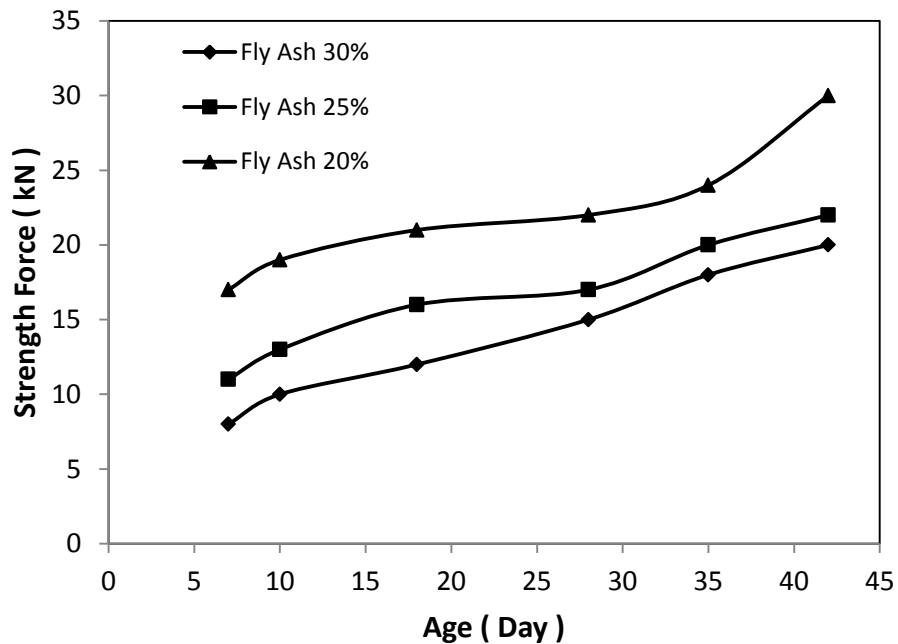
Fig.(7): The strength of concrete with aging time for calcined fly ash addition
