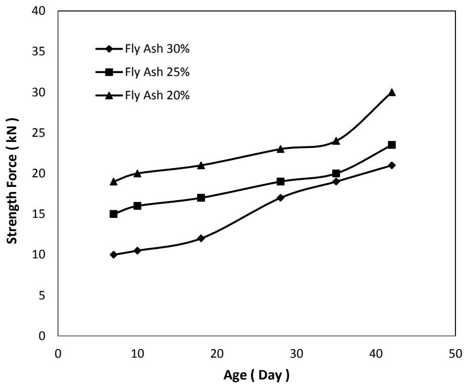
Fig.(6): The strength of concrete with aging time for fly ash addition without calcination
