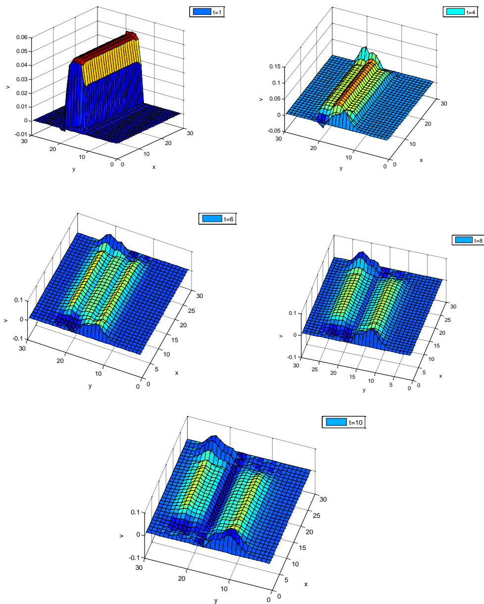
Figure 2. Solution describes the evolution of v in the system(2) for different time.
