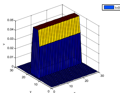
Figure 1. plot of initial data v(x, y, 0)
