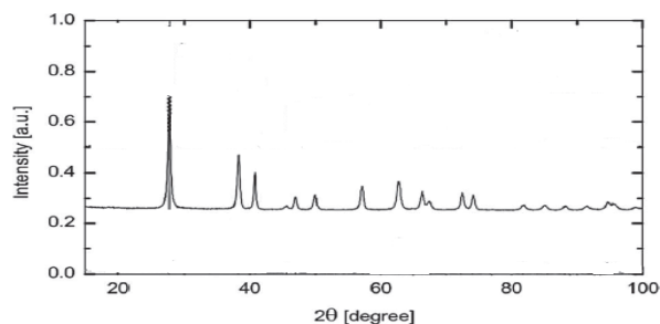
Figure (4) X-ray diffraction pattern of the thin film LiNbO 3
