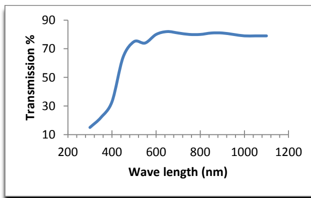
figure(6) the transmission spectrum of the LiNbO 3 thin film
