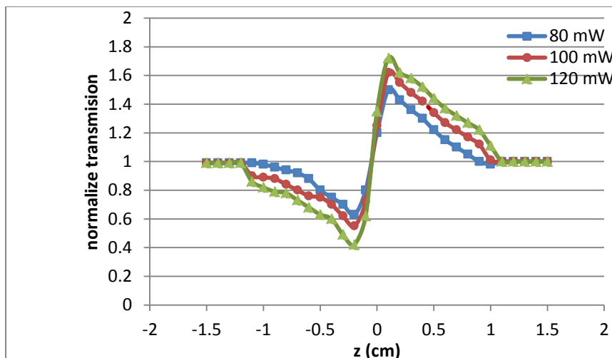
Figure (9) Closed-aperture Z-Scan at 1064 nm
