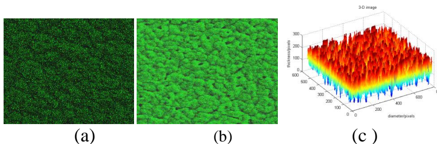
Figure (5) Thin film LiNbO 3 (a) Recording DHM (b) reconstruction DHM (c) topography of the film
