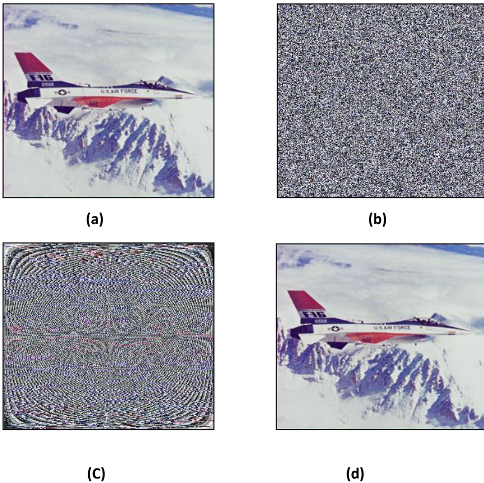
Figure ( 3 ): (a) Plain image " airplane.bmp "; (b) cipher image with no. of iterations=10; (c) decryption image with only one loop is differ=9 and (d) decryption image with same parameter and number of iterations.
