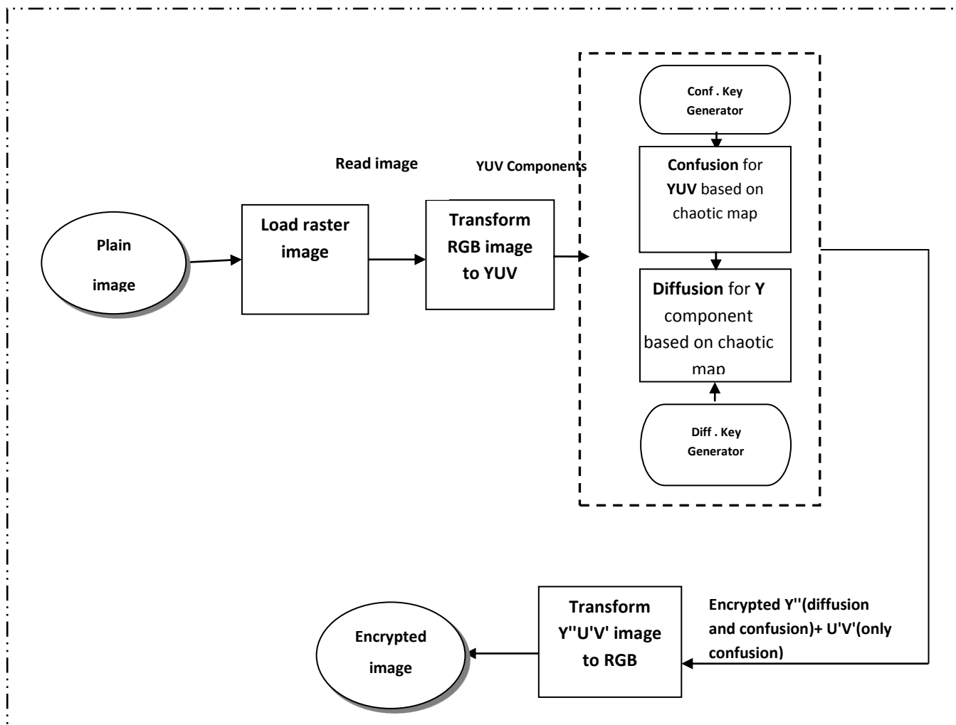
Figure (1) Encryption Module of Proposed Scheme
