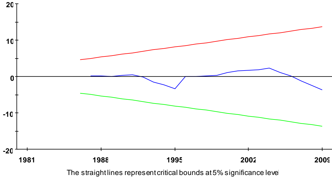
الشكل رقم (1) Plot of Cumulative Sum of Recursive Residuals
