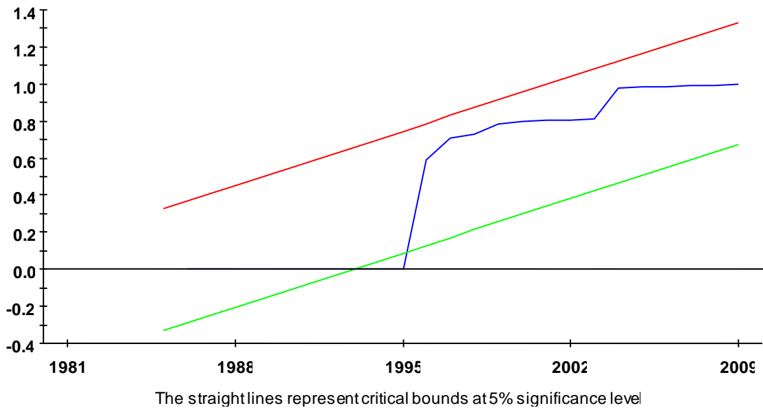
الشكل رقم (4) Plot of Cumulative Sum of Squares of Recursive Residuals
