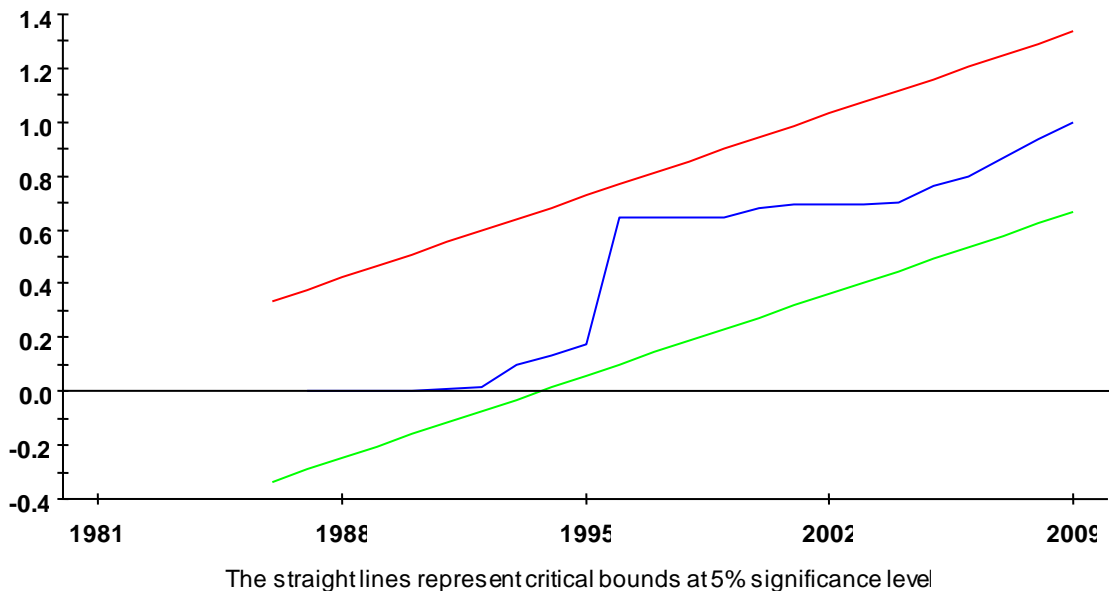
الشكل رقم (2) Plot of Cumulative Sum of Squares of Recursive Residuals
