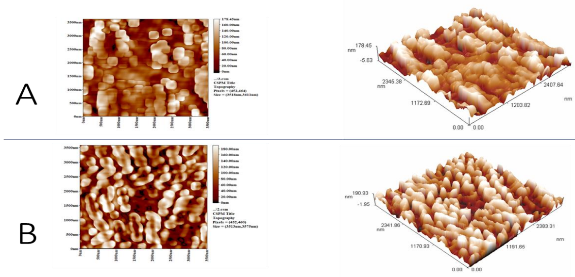
Figure 1 : AFM micrographs, 3 D and 2D graphs for the average roughness of specimen.
