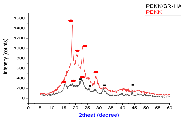
Figure (2) : XRD pattern of PEKK and PEKK coating with Sr-HA specimen
