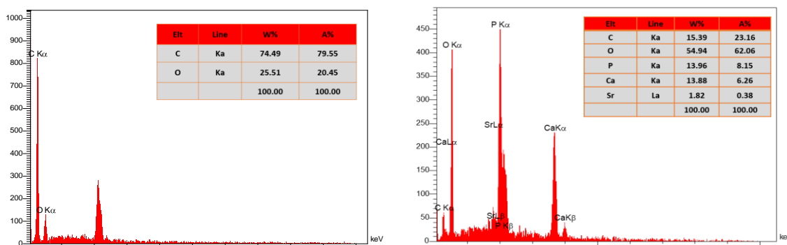
Figure (3) : EDX spectrum of PEKK and PEKK coating with SR HA specimen
