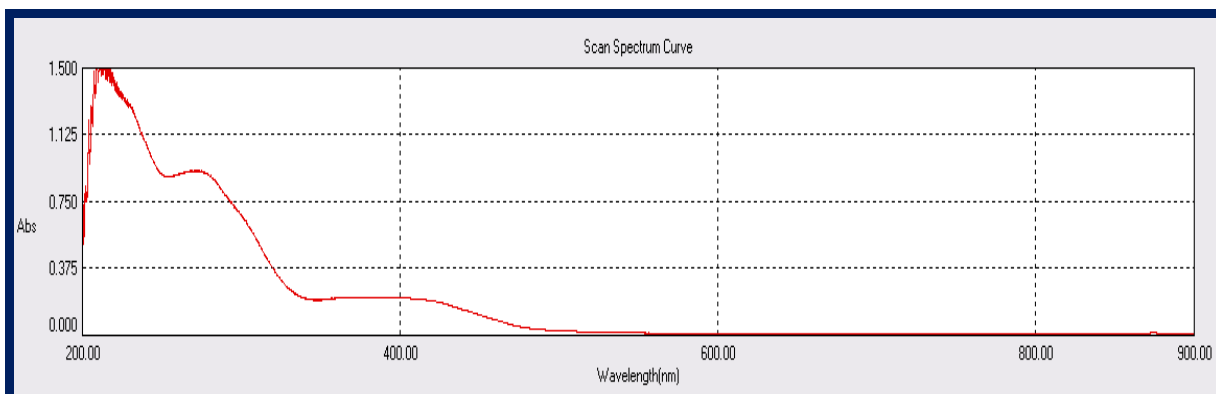
Figure 7. Absorption spectra of N-[4-Hydroxy-3-(5-mercapto-[1,3,4]thiadiazolyl-2-azo)-phenyl]-acetamide
