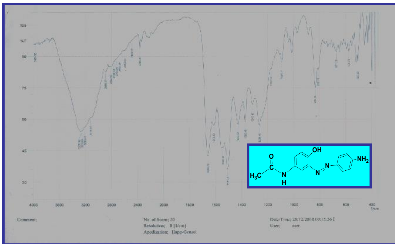
Figure (2) FTIR spectrum of N-[3-(4-Amino-phenylazo)-4-hydroxy-phenyl]-acetamide
