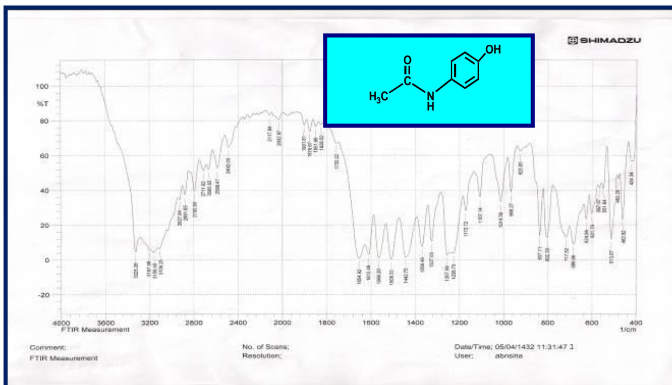
Figure (1) FTIR spectrum of paracetamol
