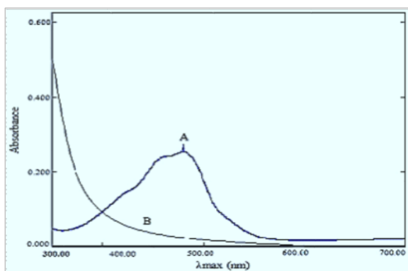
Figure 3. Absorption spectrum of the reaction A\HCTZ ( 10\mu\text{g. mL}^{-1} ) B\ blank
