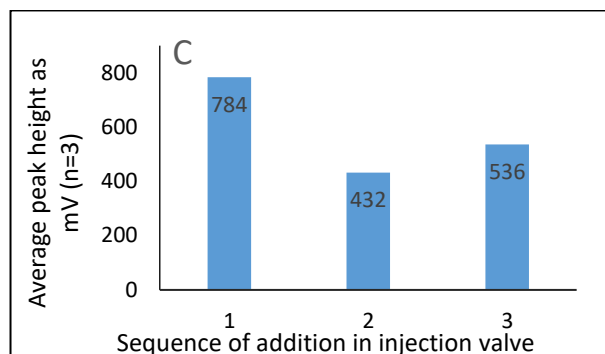
Figure 7. Effect of concentration A\ O-Ph, B\ K_3[Fe(CN)_6] , C\ sequence of chemicals.
