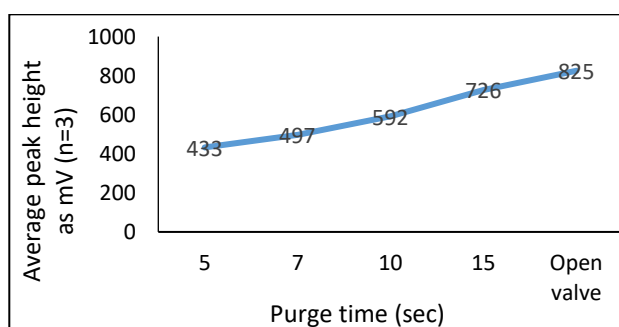
Figure 11. Effect of purge time
