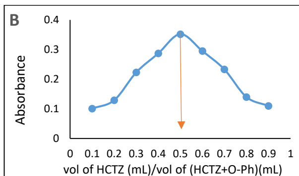
Figure 6. Stoichiometric ratio of drug to the reagent (a) Mole ratio (b) Continuous variation
