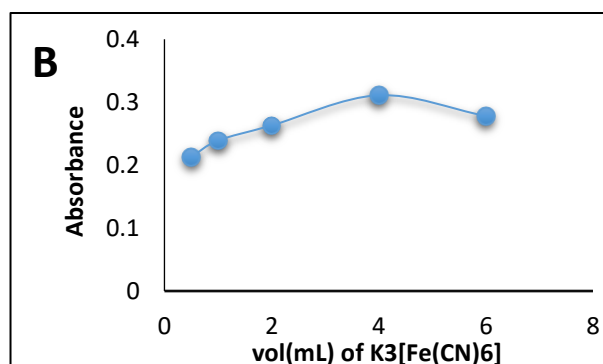
Figure 4. Effect A/ volume of O-Ph, B/ volume of \text{K}_3[\text{Fe}(\text{CN})_6]
