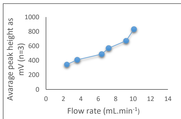
Figure 8. Effect of flow rate in a developed system
