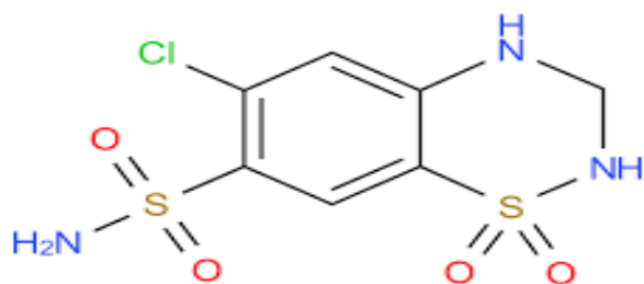
Figure 1. Formula structure of HCTZ 10 .
