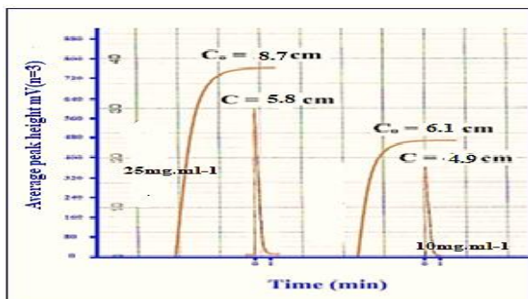
Figure 12. Dispersion of HCTZ in CFIA system.
