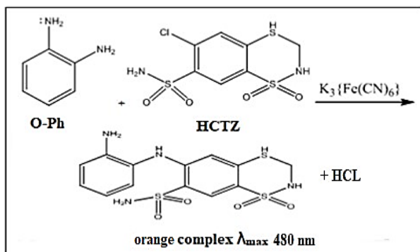
Scheme 1. The pathway of reaction for HCTZ and O-Ph.
