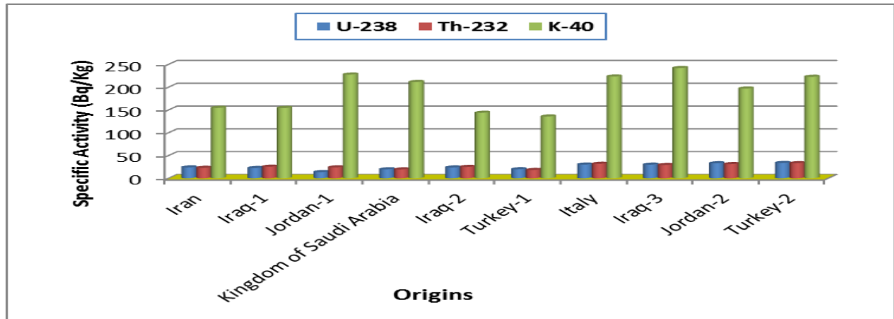
Fig.(1): specific activity of ( ^{238}\text{U} , ^{232}\text{Th} and ^{40}\text{K} ) for all phosphate fertilizers samples.
