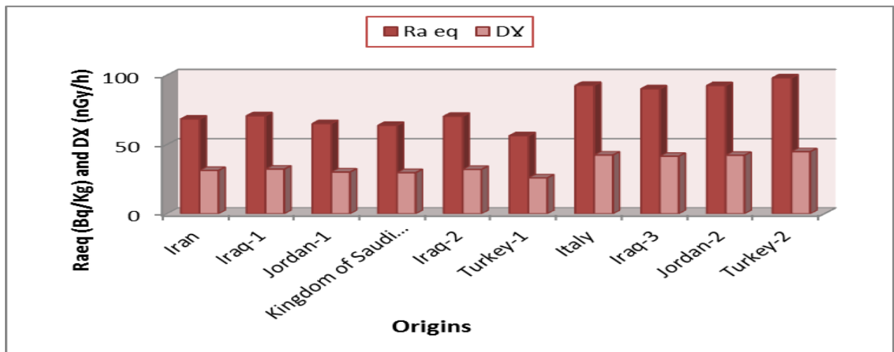
Fig.(2): equivalent activity of radium and dose rate of absorbed gamma for all phosphate fertilizers samples.
