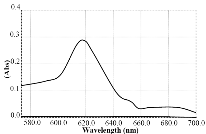
Fig. 2: Absorption spectrum of Capoten-Nickel(II) complex.
