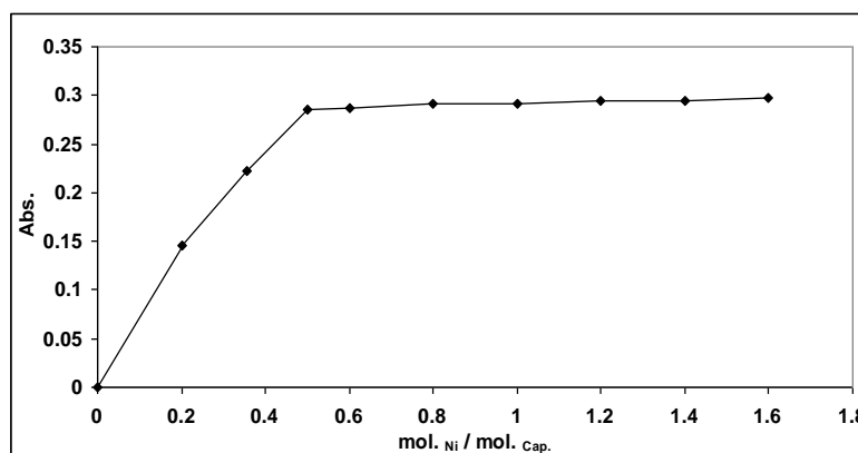
Fig. 10: molar ratio plot for Capoten-Nickel(II) complex ratio.
