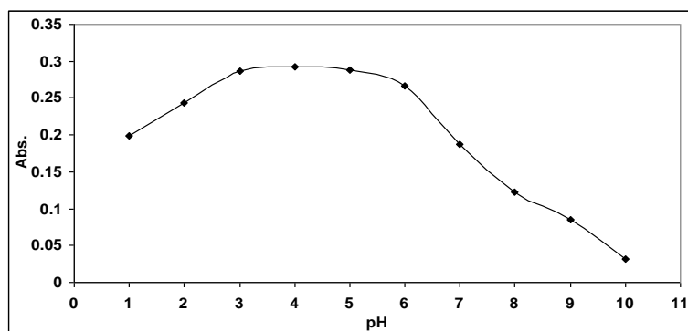
Fig. 5: Effect of pH on the absorbance of Capoten-Nickel(II) complex.
