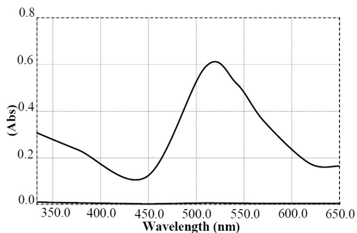
Fig. 4: Absorption spectrum of Ni(NO 3 ) 2 .6H 2 O.
