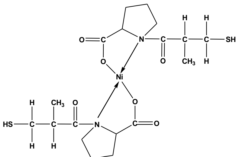
Scheme 1: The proposal structure of Capoten-Nickel(II) complex.
