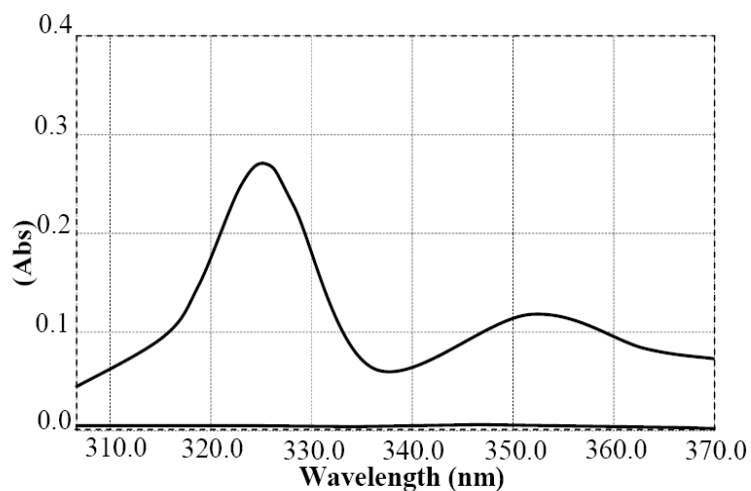
Fig. 3: Absorption spectrum of Capoten.
