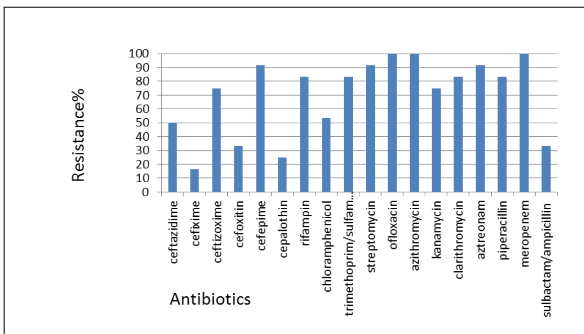
Fig.1 Antibiotic susceptibility of Aeromonas hydrophila isolated from patients with diarrhea.
