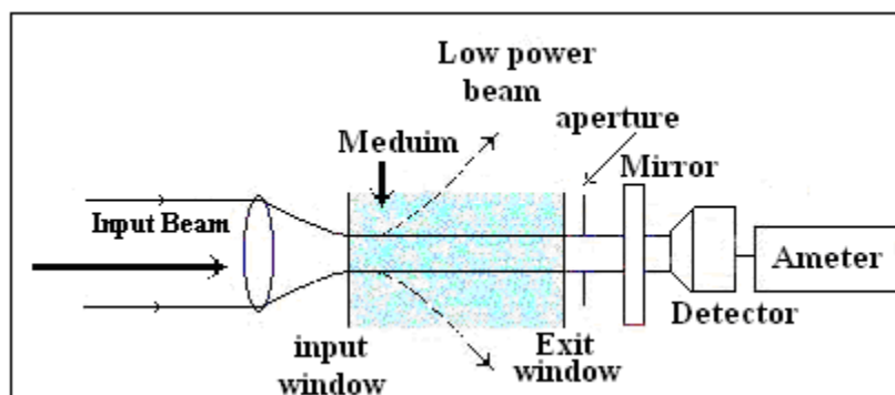
Figure (1): Schematic diagram of the bistable optical device.
