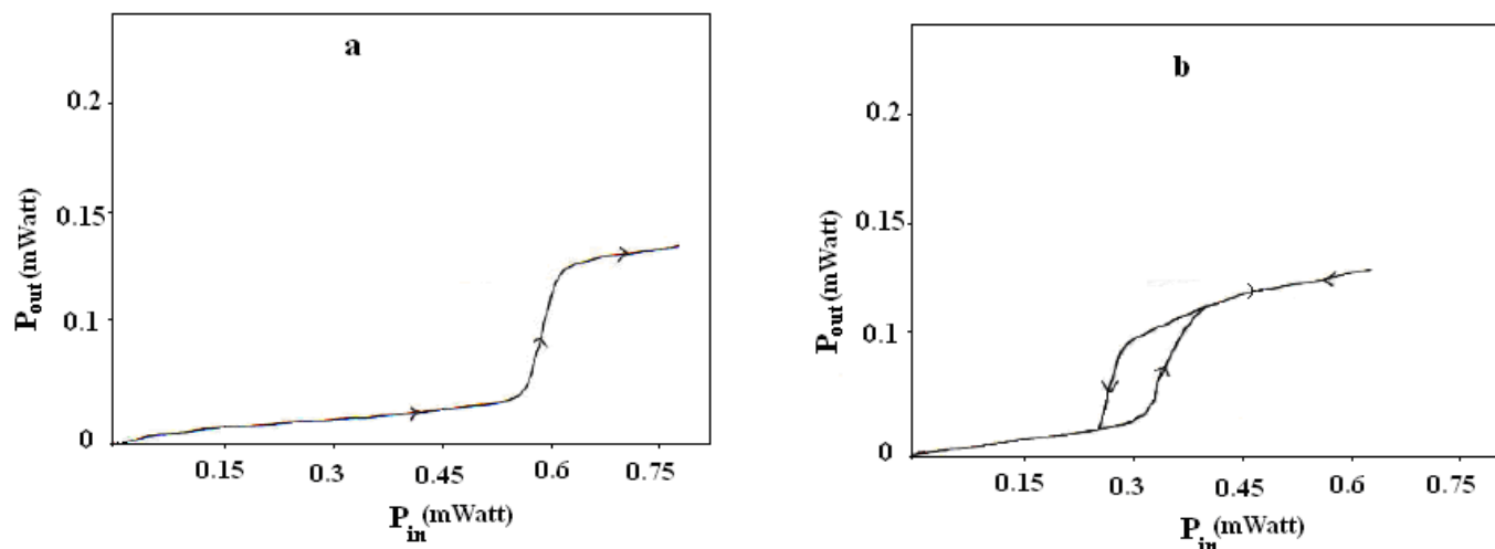
Figure (2): Experimental curve of P_{out} versus P_{in} (a) without the mirror showing the optical limiting mode of the mirrorless situation. (b) With the mirror in place so that the device exhibits bistable operation.
