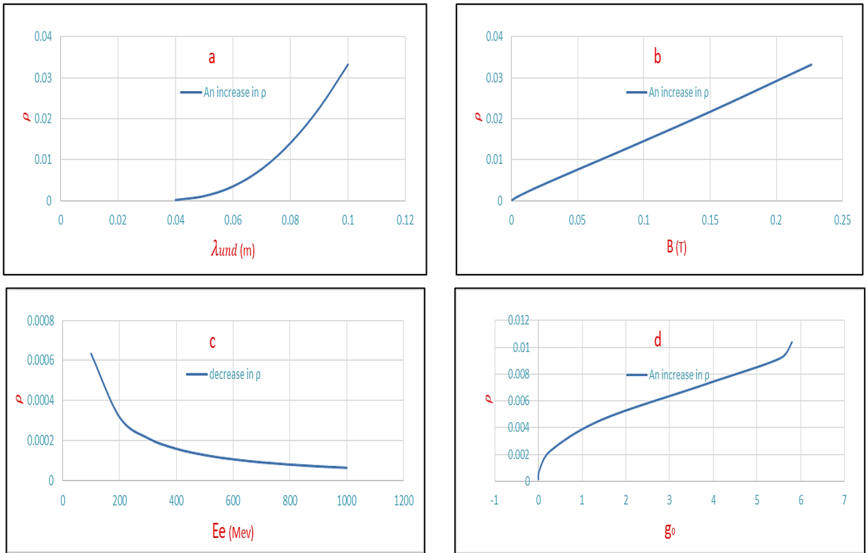
Figure 3: The relations between \rho versus ( \lambda_{und} , B , E_e , g_0 )
