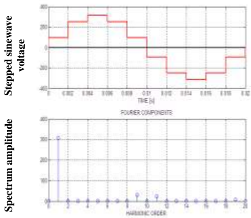
Fig(7):The Spectrum analysis of three and five nonzero stepped sine wave signal
