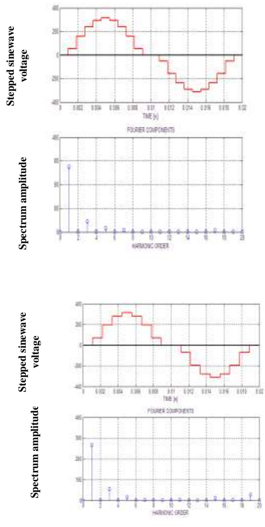
Fig (5): The spectrum analysis of seven and nine steps zero crossing sine wave signal
