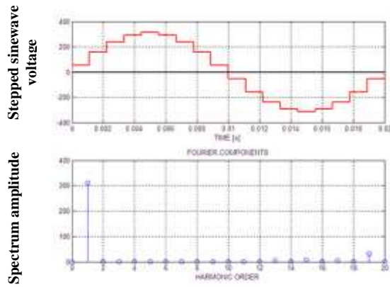
Fig (8):The spectrum analysis of seven and nine Steps non zero crossing sine wave
