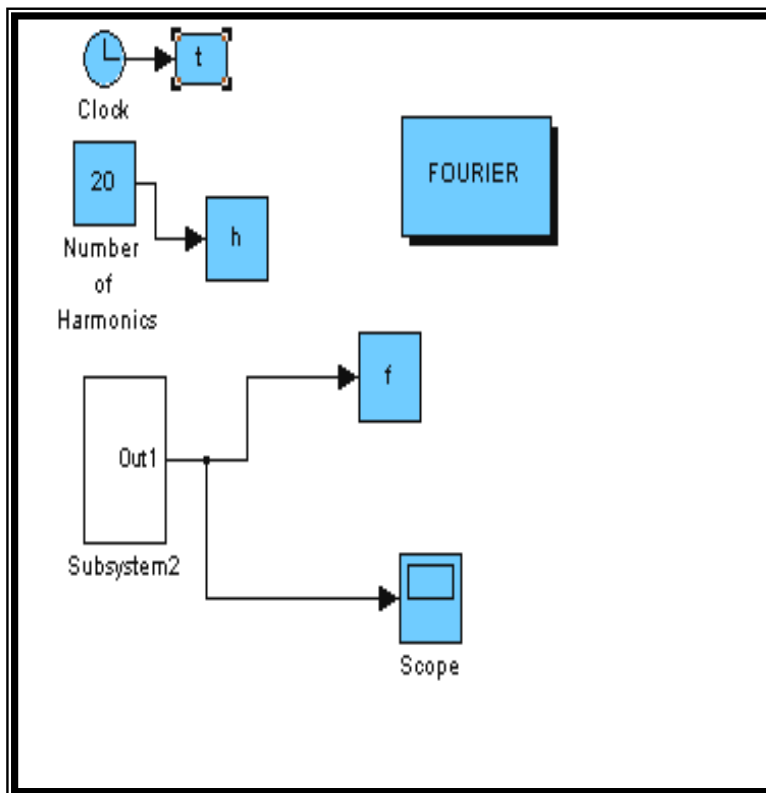
Fig(3):Simulated diagram for stepped sinewave signal
