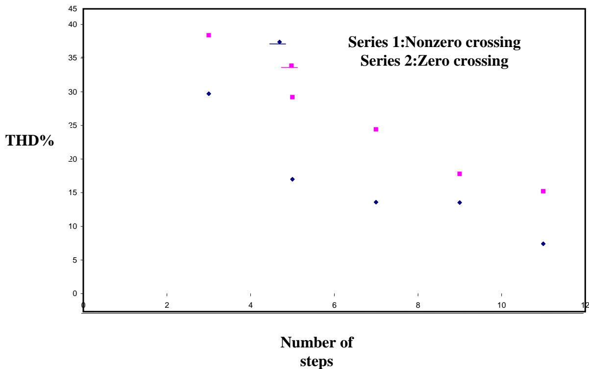
Fig(10): Comparison between zero crossing and nonzero crossing stepped signal with THD%
