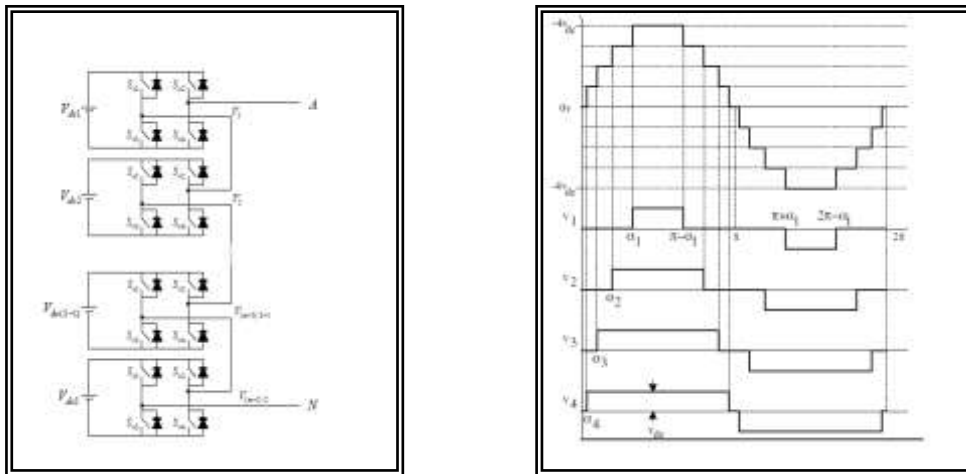
Fig. (1) : (a)Single- phase structure of a m-level cascaded inverter. (b) Output Voltage Waveform of the H-bridge Cell series-connected Cascaded Multilevel Inverter
