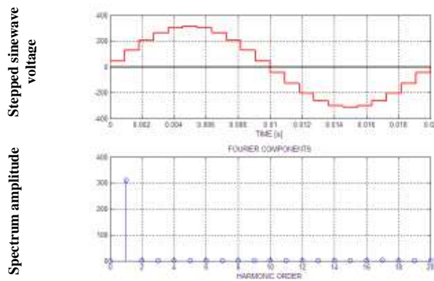
Fig (9):The spectrum analysis of eleven Steps non zero crossing sine wave
