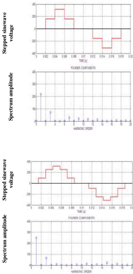
Fig (4):The spectrum analysis of three and five steps zero crossing sine wave signal
