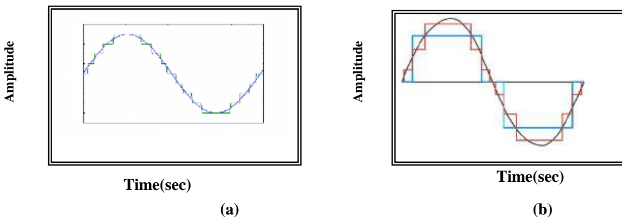
Fig. (2). (a)Zero crossing stepped sinewave (b) Nonzero crossing stepped sinewave
