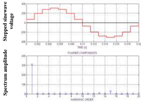
Fig (6):The spectrum analysis of Eleven Steps zero crossing sine wave
