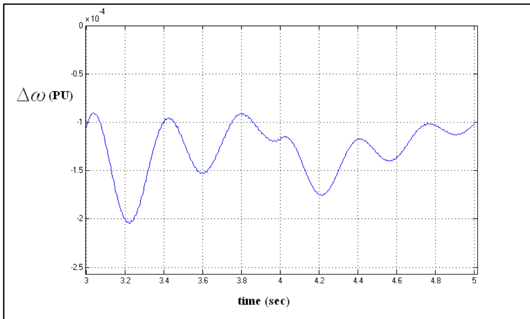
Fig. 9. The speed deviation for a step change in the reference voltage
