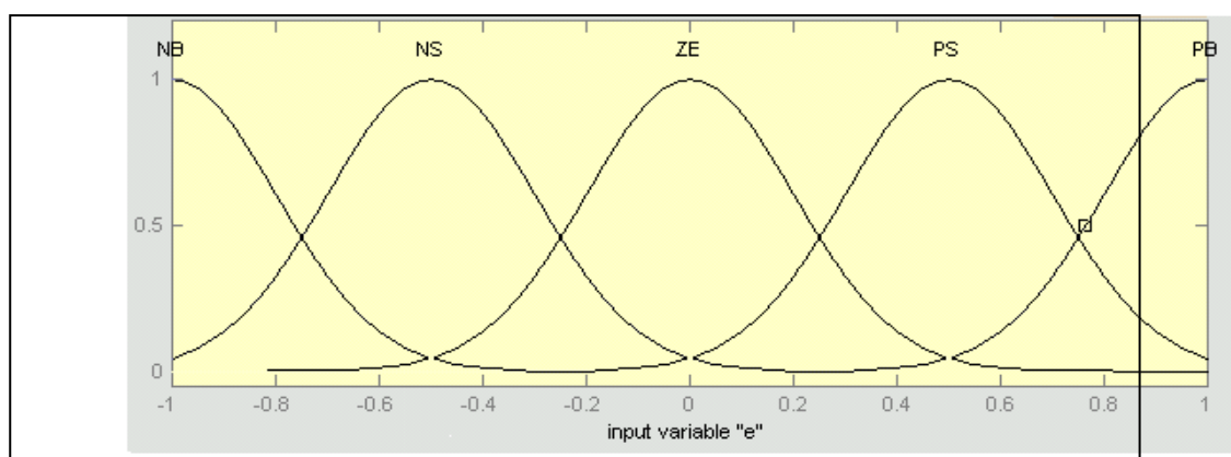
Fig. 5. The membership functions of input linguistic terms.
