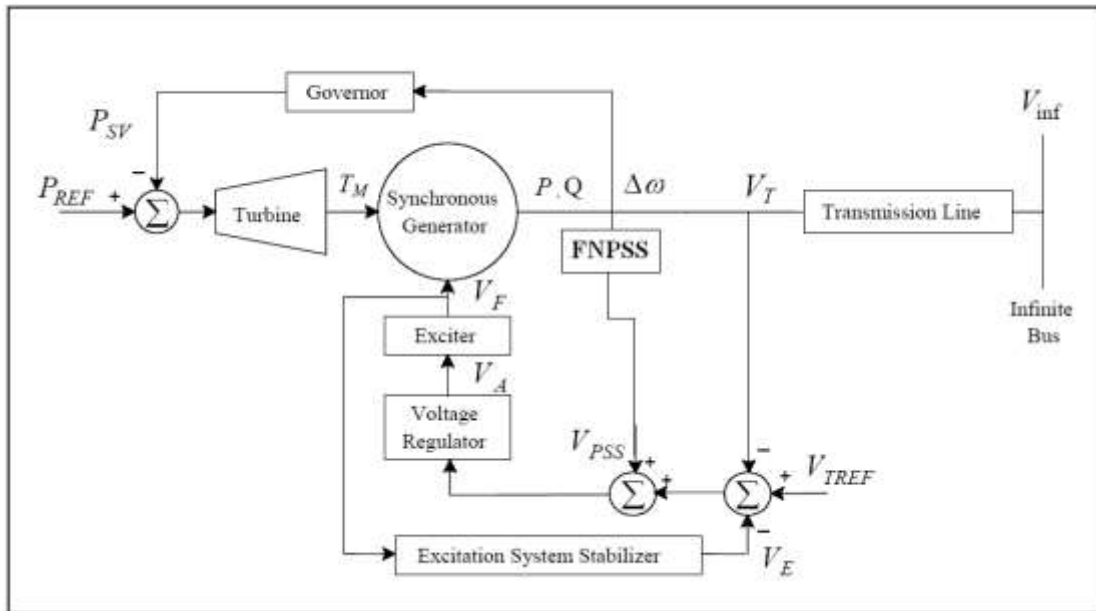
Fig. 1. System model configuration
