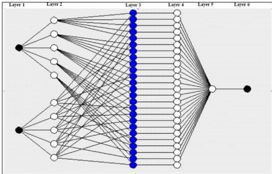
Fig.7. The ANFIS structure.
