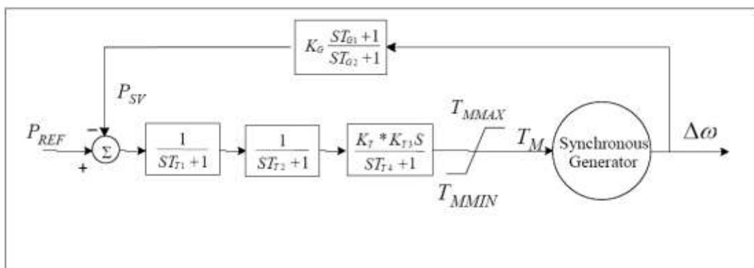
Fig. 2. Block diagram of the turbine and the governor
