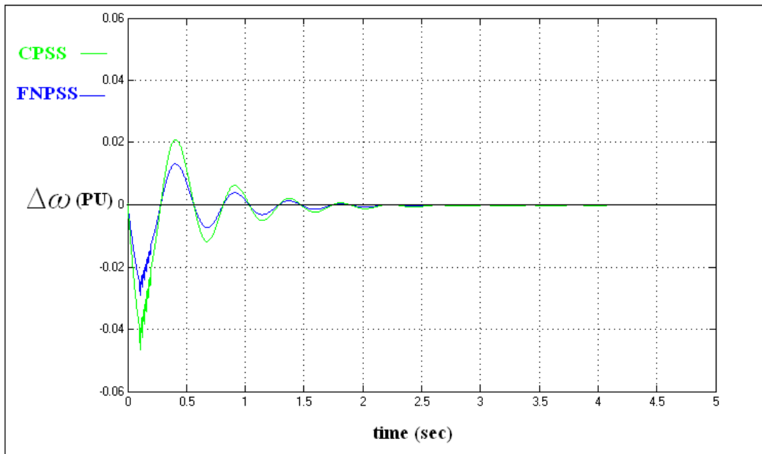
Fig. 8. The speed deviation (PU) for a fault at the bus
