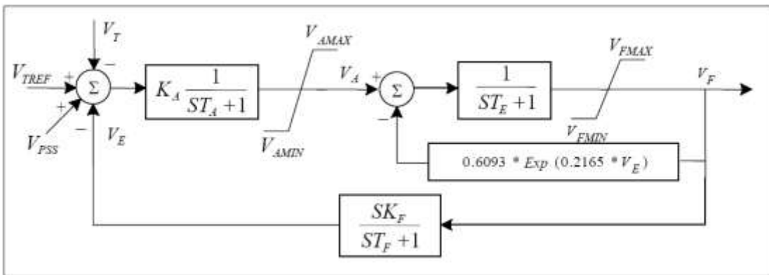
Fig. 3. Block diagram of the excitation system
