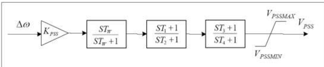
Fig. 4. Block diagram of the conventional power system stabilizer
