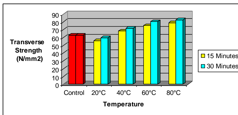
Figure (1): Bar chart for transverse strength mean values of control and specimens polymerized at different curing times and water temperatures.
