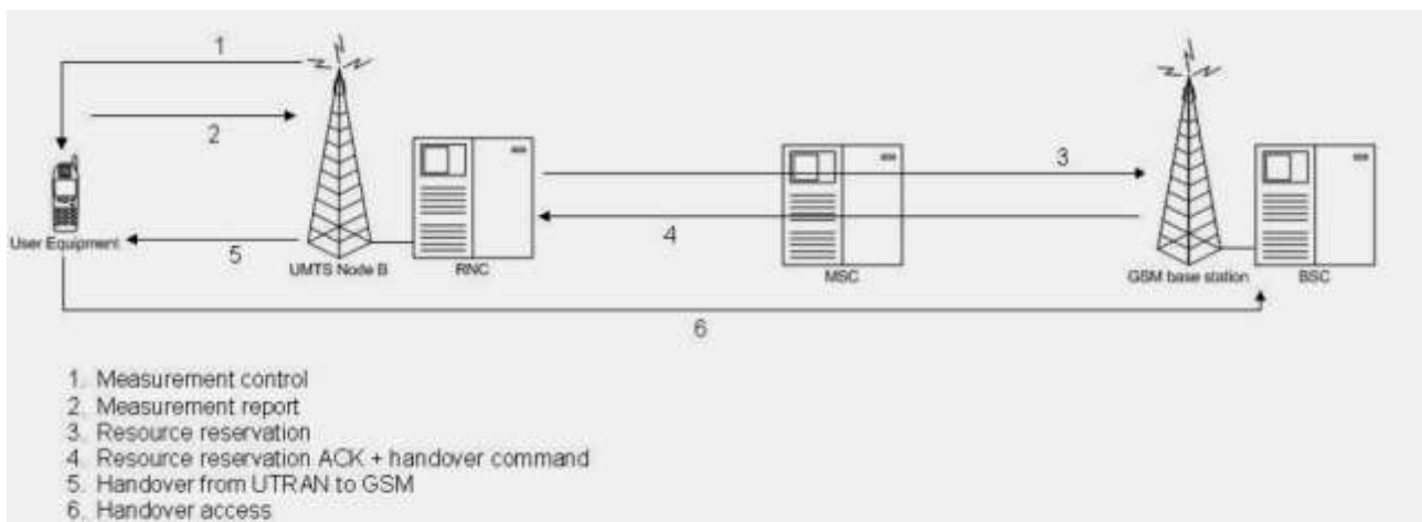
Figure 2 Inter-system handover procedure from UTRAN to GSM
