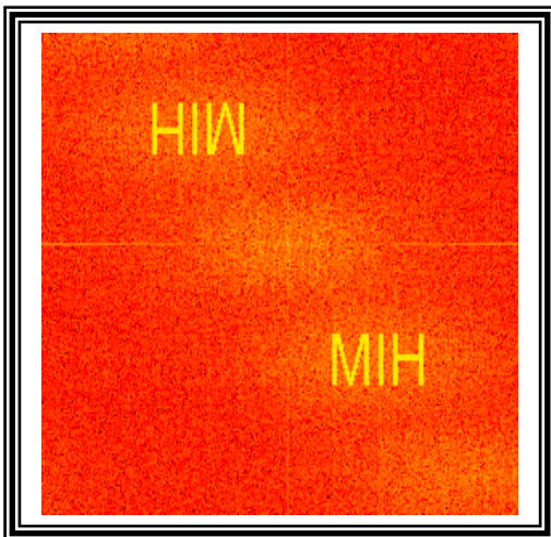
Fig(10): Digital reconstruction image of a hologram with random phase and expansion the scale of sampling.
