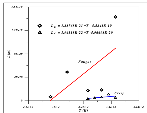
Fig(7) shows the temperature effect in a crack propagation length per one step of activation energy for a creep and the fatigue crack propagation.
