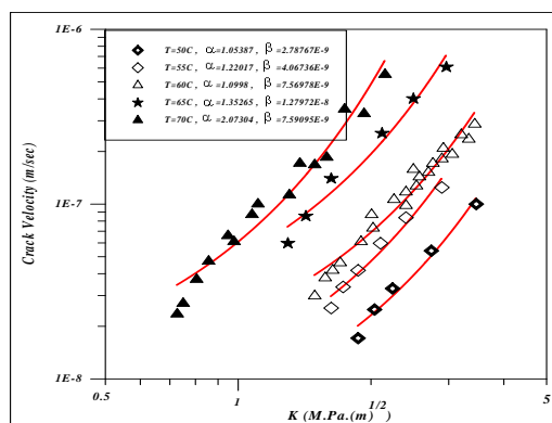
Fig (3): shows (EFP) of (V- \Delta K ) plot for creep crack propagation in PVC tubes with different temperature degrees.
