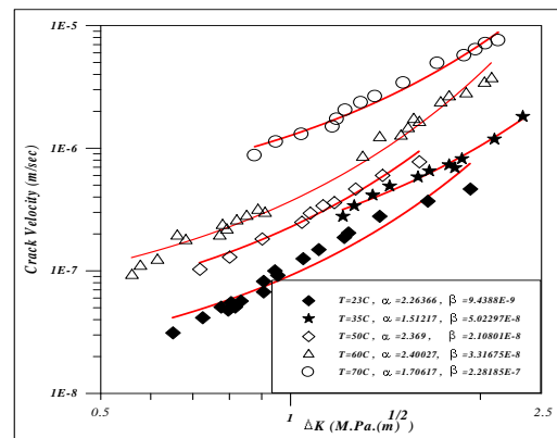
Fig (4) shows (EFP) of (V- \Delta K )plot for fatigue crack propagation in PVC tubes with different temperature degrees .
