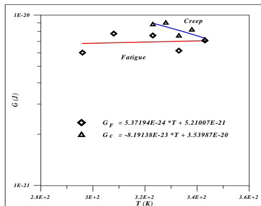
Fig (6) shows the temperature effect in the surface energy for a creep and the fatigue crack propagation
