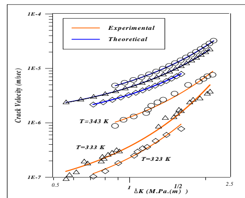
Fig (9) shows the comparative between experimental data of crack velocity and theoretical crack velocity in eq(3-8).
