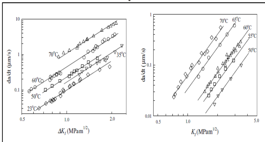
Fig(1): shows the effect of temperature on the (V-K, \Delta K ) plots for creep and fatigue crack propagation in PVC pipes[5]
