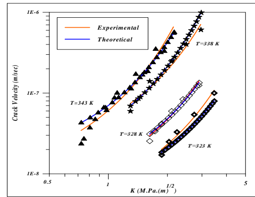
Fig (8) shows the comparative between experimental data of crack velocity and theoretical crack velocity in eq(3-7) .
