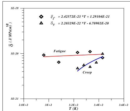
Fig(5) shows the temperature effect in the work constants for a creep and the fatigue crack propagation.
