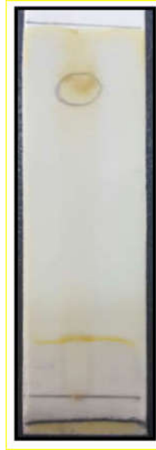
Figure 1: Thin layer chromatography for isolated alkaloid
