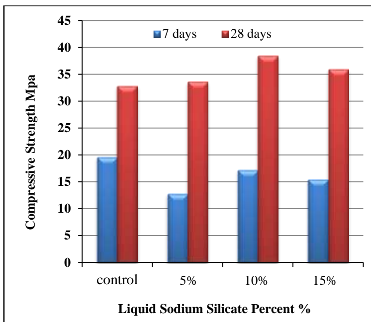
Figure (4) : Effect of Liquid Sodium Silicate percent on compressive strength
