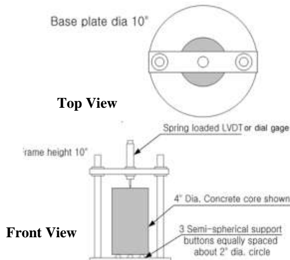
Figure (2) Schematic of a Measuring Frame (AASHTO TP 60 2004) [15]
