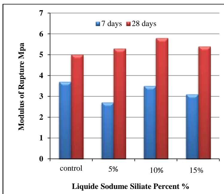
Figure (5) : Effect of liquid Sodium Silicate percent on modulus of rupture
