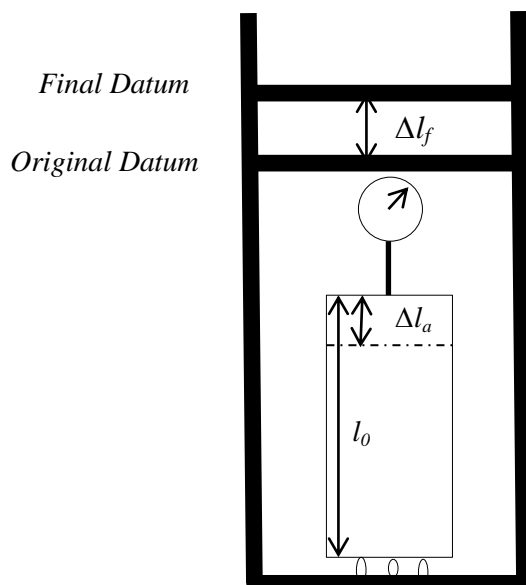
Figure (3): Schematic of the CTE test frame (Drawing not to Scale)
