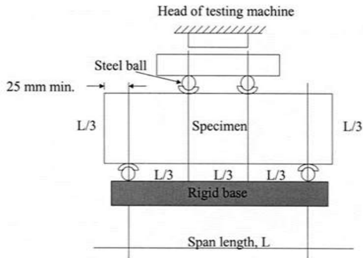
Figure (1) : Test for modulus of rupture
