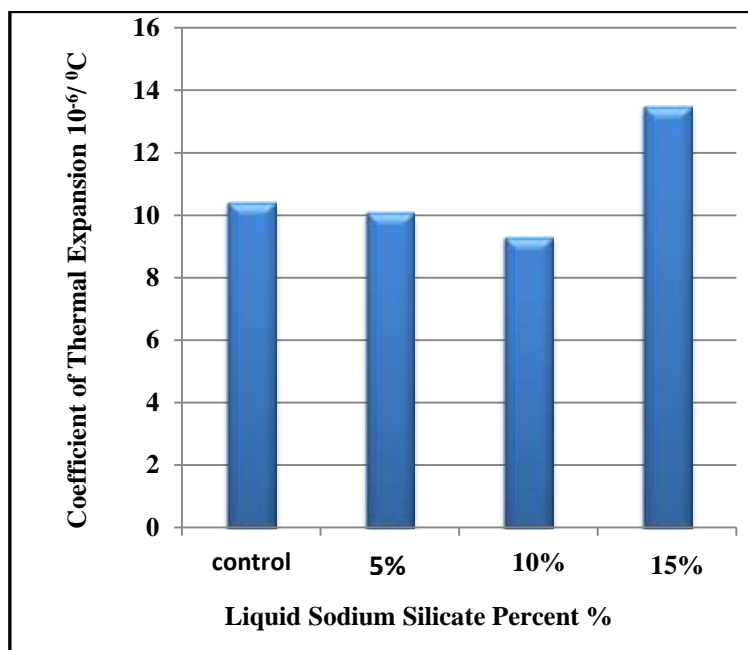
Figure (6) : Effect of liquid Sodium Silicate percent on coefficient of thermal expansion for samples aged 28 days
