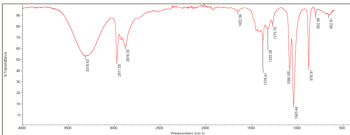
Figure 15. IR spectrum of chelidonium.
