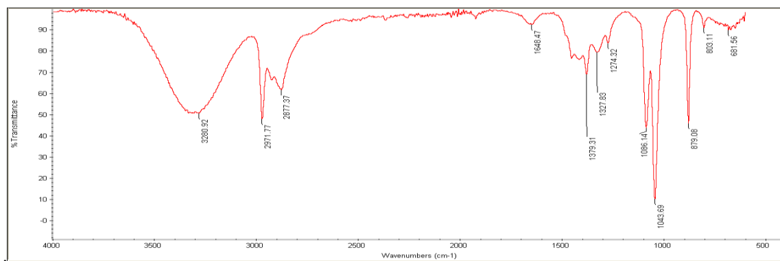
Figure 11. IR spectrum for compound B
