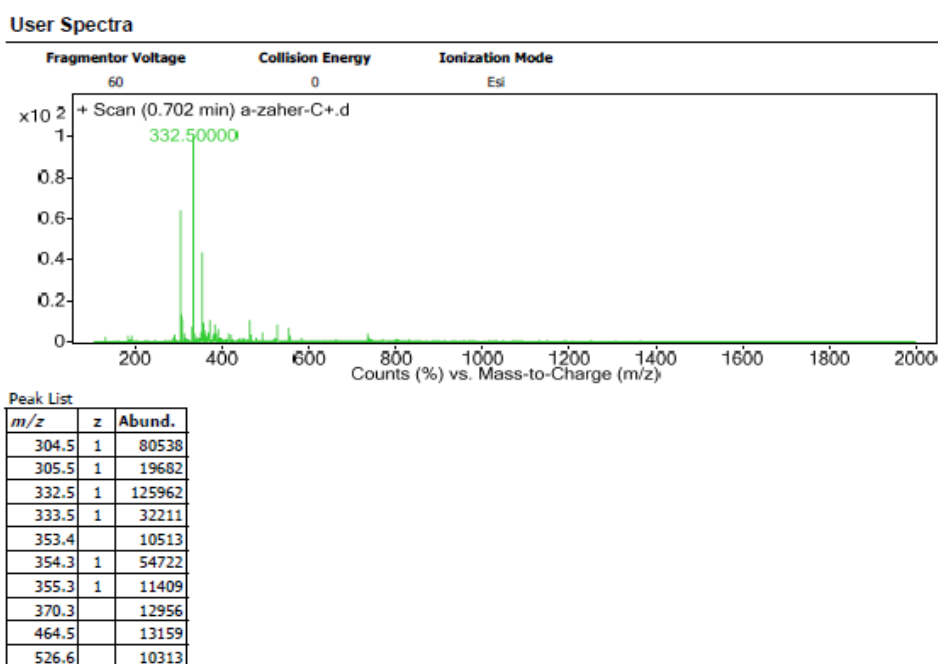
Figure 4. LC mass for compound A.
