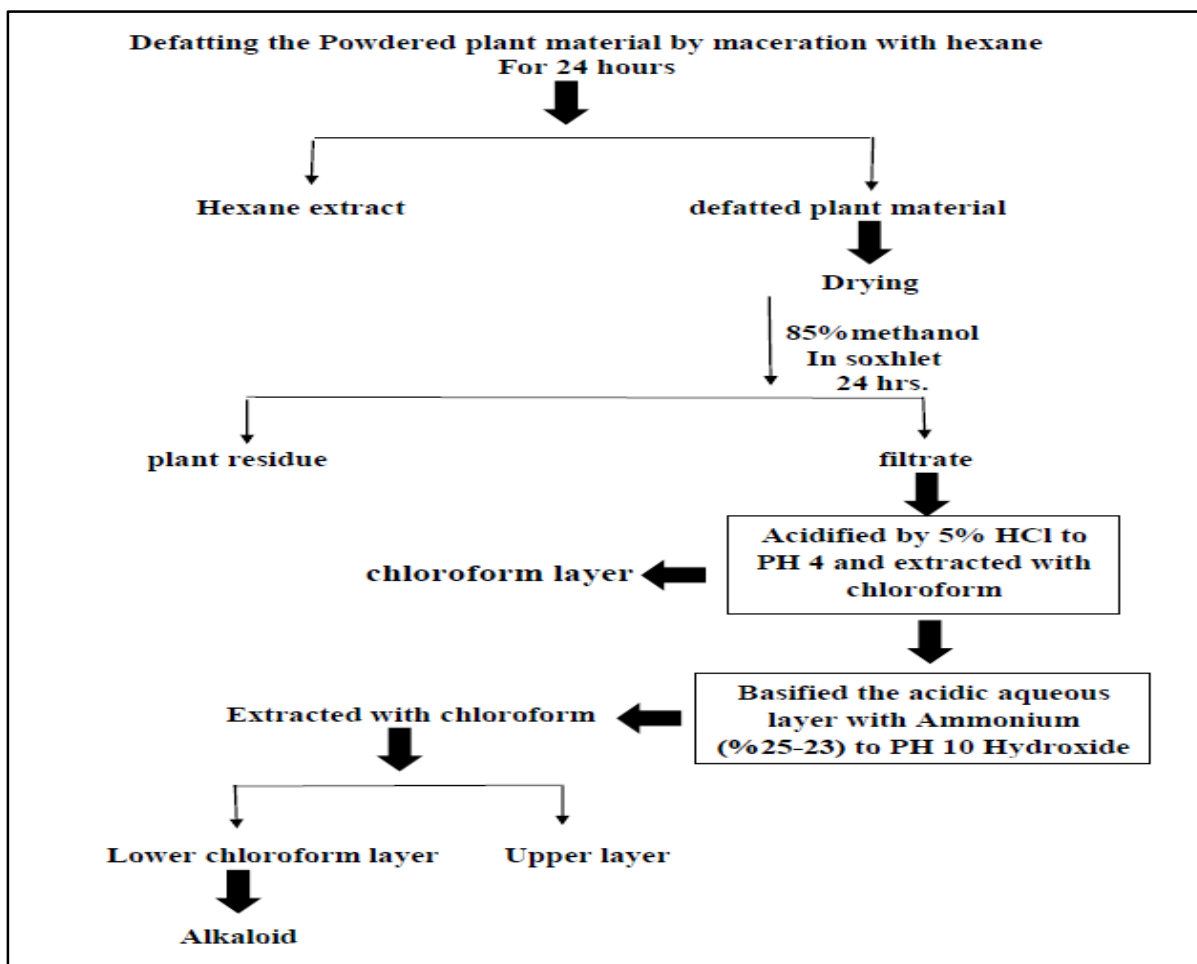
Figure 2. Steps of alkaloids extraction.
