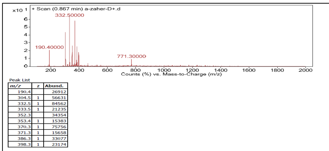
Figure 8. LC mass for compound B.
