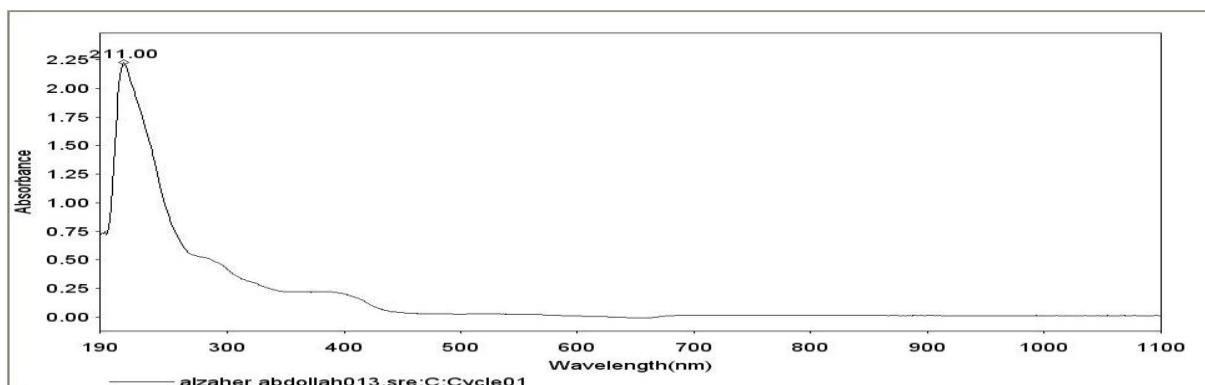
Figure 6. The \lambda max spectrum for dihydrocodeine.
