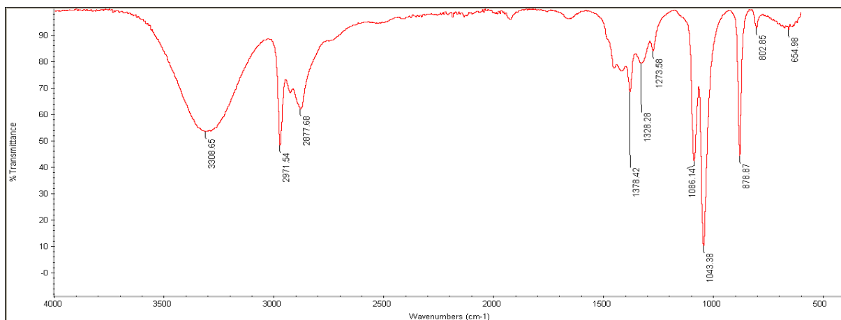
Figure 7. IR spectrum for compound A
