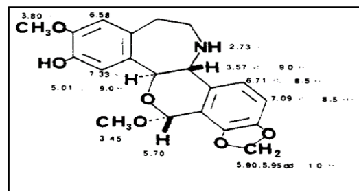
Figure 9. chemical structure of compound B indicated Papaverrubine C (Epiporphyroxine).
