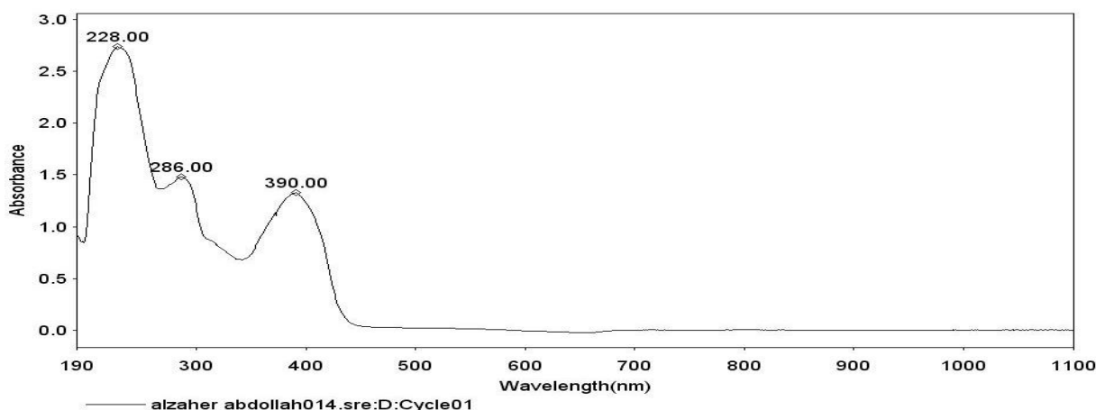
Figure 10. The \lambda_{max} spectrum for Papaverrubine C compound.
