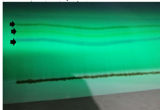
Figure 3. Preparative TLC chromatogram for Papaver rhoeas alkaloids on silica G F254 plate using mobile phase Cyclohexane: Chloroform: Diethylamine (70:20:10) under U.V light
