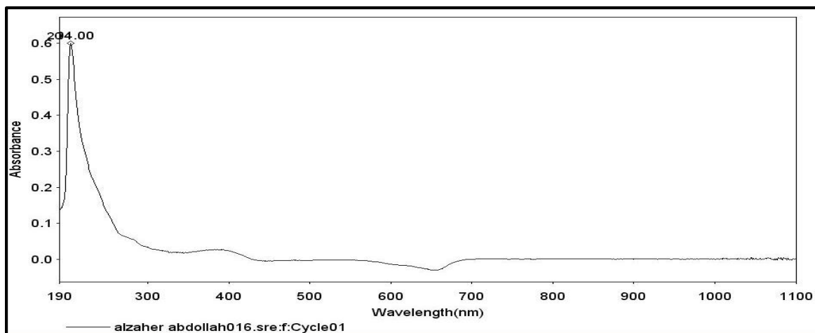
Figure 14. The \lambda max spectrum for compound C
