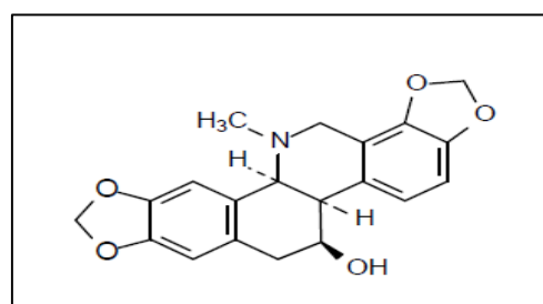
Figure 13. chemical structure of chelidonium.
