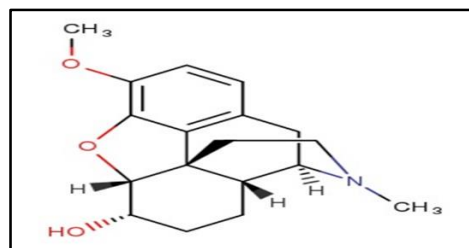
Figure 5. Chemical structure of compound A (dihydrocodeine).
