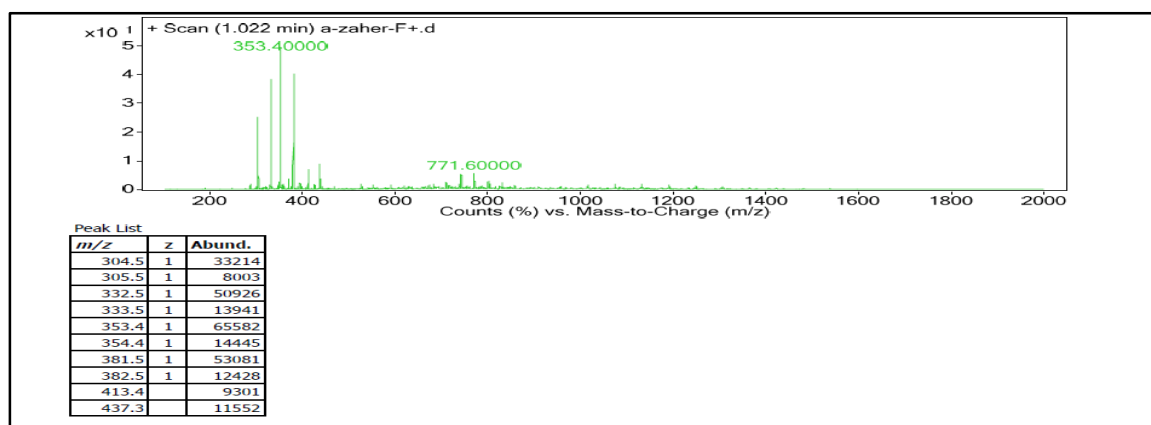
Figure 12. Lc mass diagram for compound C.
