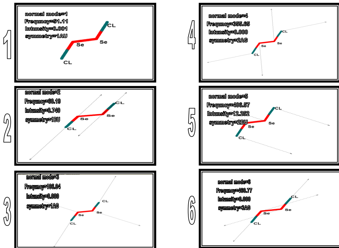
Fig(2) Vibrational Modes of [\text{Se}_2\text{Cl}_2]
