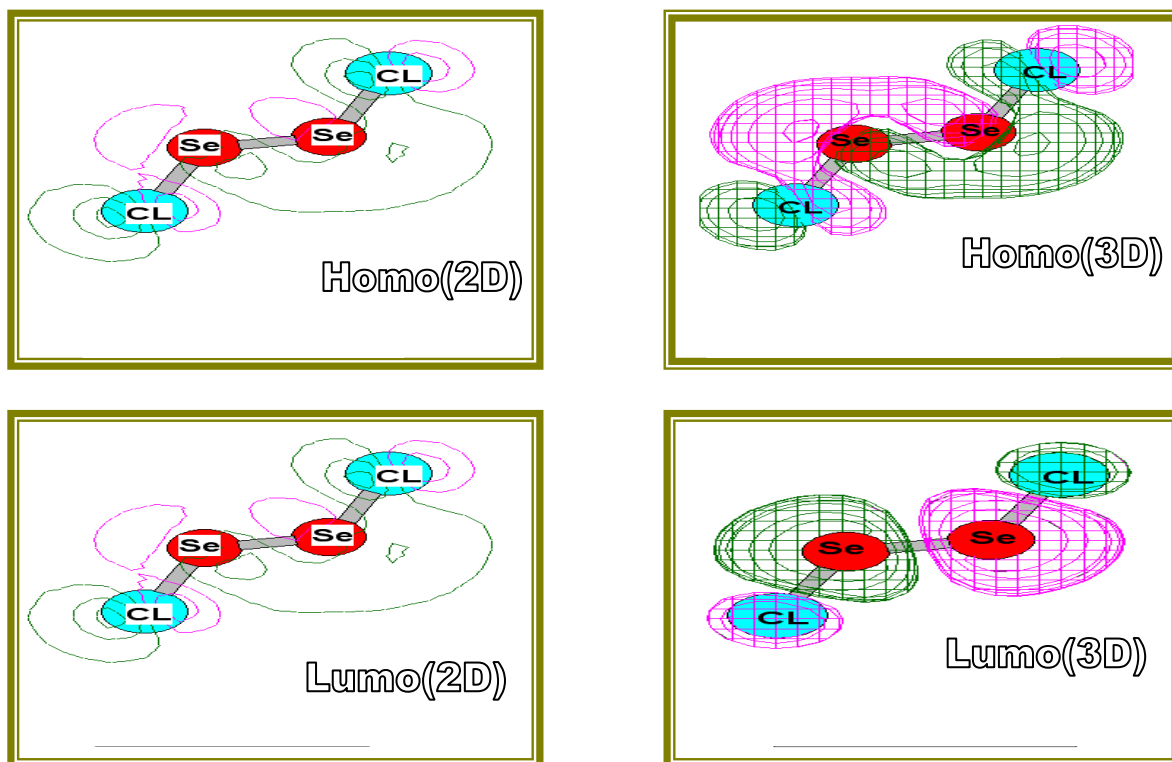
Fig(4) Energy level of Homo & Lumo of ( \text{Se}_2\text{Cl}_2 ) in ( 2D and 3D)
