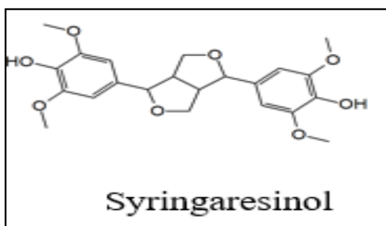
Figure 5. Chemical structure of syringaresinol (lignin) (44) .
