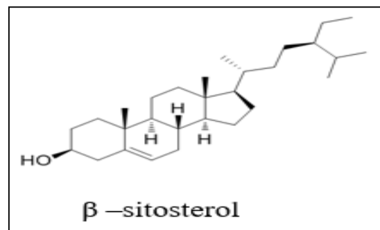
Figure 6. Chemical structure of \beta -sitosterol(phytosterol) (47) .
