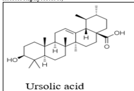
Figure 7. Chemical structure of ursolic acid (pentacyclic triterpenoids) (48) .
