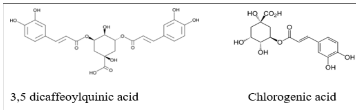
Figure 3. Chemical structures of phenolic acids (3,5-dicaffeoylquinic acid and chlorogenic acid) (39, 40) .
