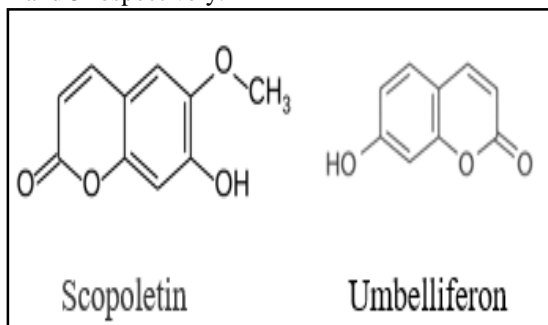
Figure 4. Chemical structure of some coumarines (scopoletin and umbelliferon) (42,43)
