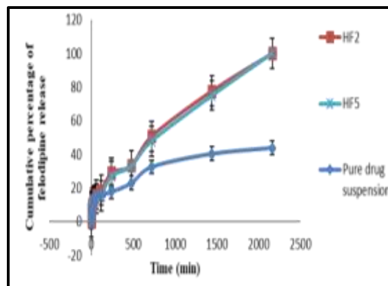
Figure 2. In vitro felodipine release profile from LPHNs formulations HF2, HF5 and the pure drug at HCl buffer pH 1.2 + 0.3 % polysorbate 80 solutions, the values of mean \pm SD (n=3).
