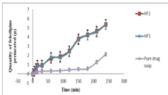
Figure 8. Permeation of felodipine from LPHNs formulations HF2, HF5 and pure drug suspension through non-everted sheep intestine, the values of mean \pm SD (n=3).
