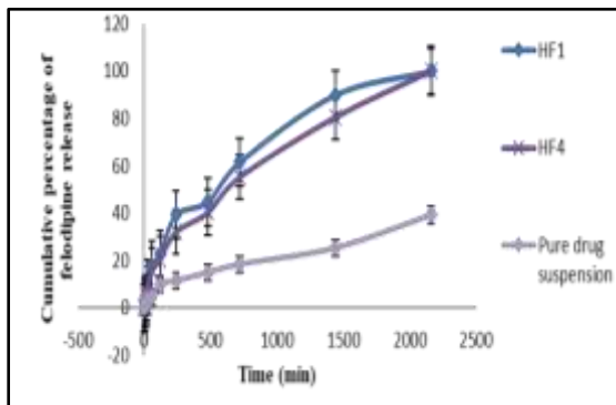
Figure 4. In vitro felodipine release profile from LPHNs formulations HF1, HF4 and the pure drug suspension at phosphate buffer pH 6.8 + 0.3 % polysorbate 80 solutions the values of mean \pm SD (n=3).
