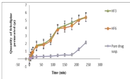
Figure 9. Permeation of felodipine from LPHNs formulations HF3, HF6 and pure drug suspension through non-everted sheep intestine, the values of mean \pm SD (n=3).
