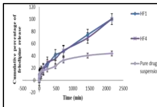
Figure 1. In vitro felodipine release profile from LPHNs formulations HF1, HF4 and the pure drug at HCl buffer pH 1.2 + 0.3 % polysorbate 80 solutions, the values of mean \pm SD (n=3).
