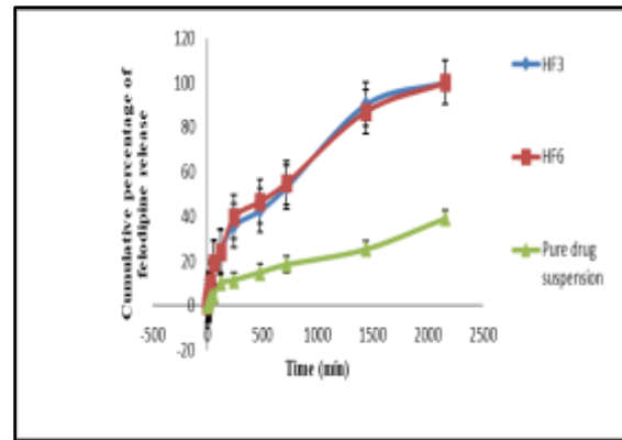
Figure 6. In vitro felodipine release profile from LPHNs formulations HF3, HF6 and the pure drug suspension at phosphate buffer pH 6.8 + 0.3 % polysorbate 80 solutions.
