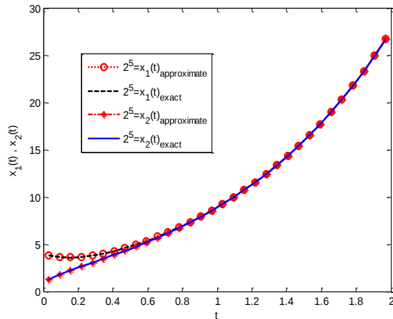
Figure 1. State space variables x_1(t) and x_2(t) for Haar wavelet resolutions m = 2^5 and t = 2 obtained from Example 1
