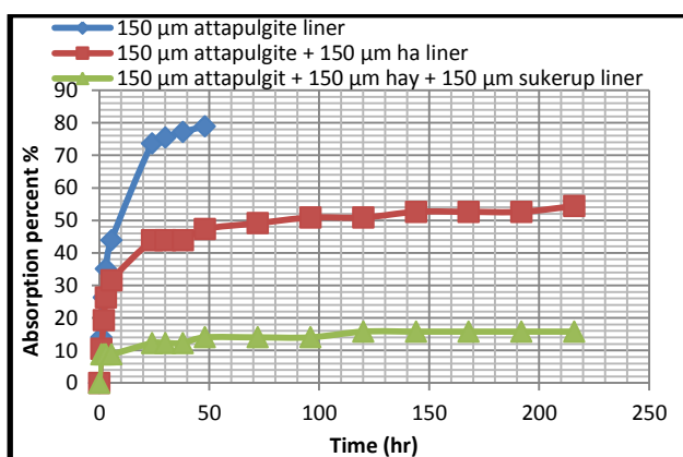
Figure 6. Attapulgitite liner mixed with prairie hay and coconut husk tested with light crude oil.
