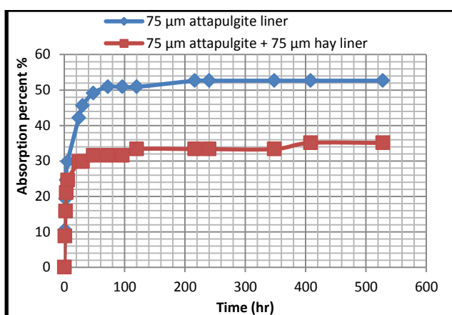
Figure 7. Liner attapulgitite 75µm and liner attapulgitite75µm mixed with prairie hay 75µm tested with light crude oil.
