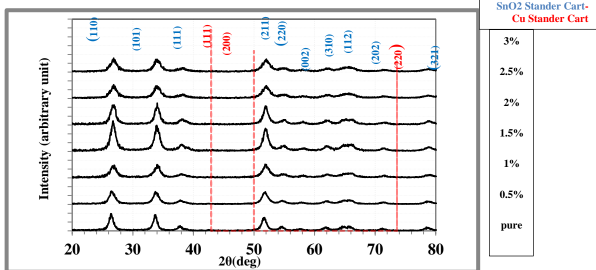
Figure. 1 X-ray diffraction pattern of pure SnO 2 nanoparticles doped with concentrations (0.5, 1, 1.5, 2, 2.5, and 3) %wt of Cu.
