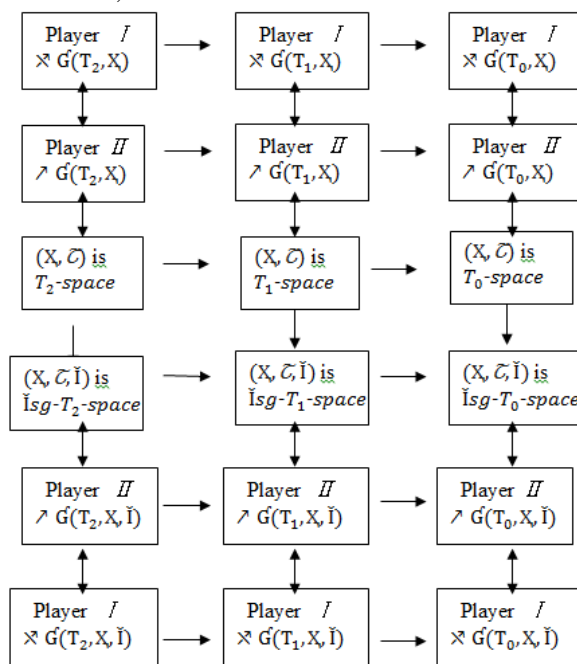
Scheme 2. Diagram of the implication in Remark 3.
