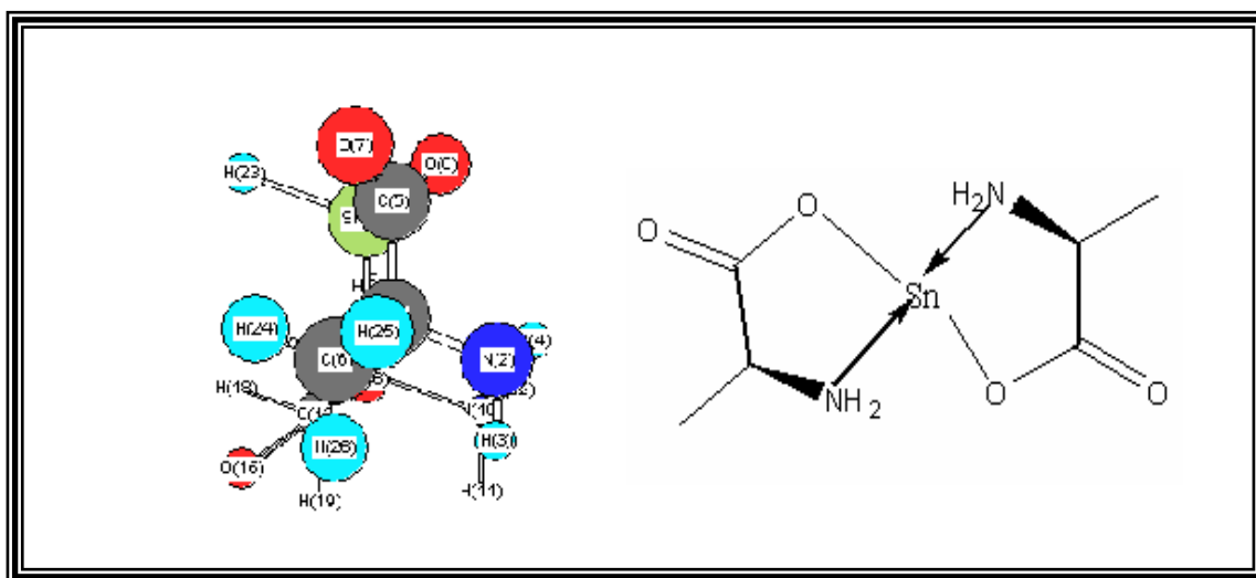
Fig (1) : The proposed molecular structure of the [\text{Sn} (\text{Ala-H})_2] .
