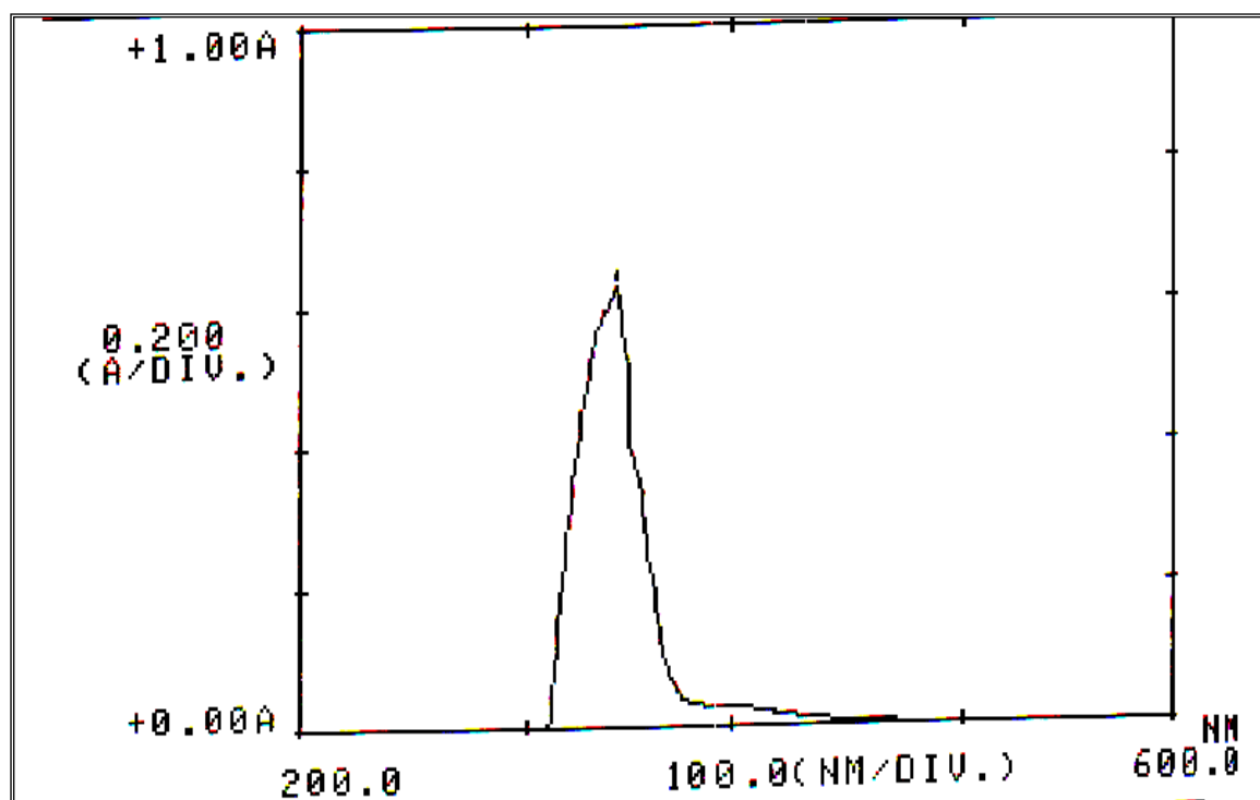
Fig(٤) Uv –Vis Alaninate ion
