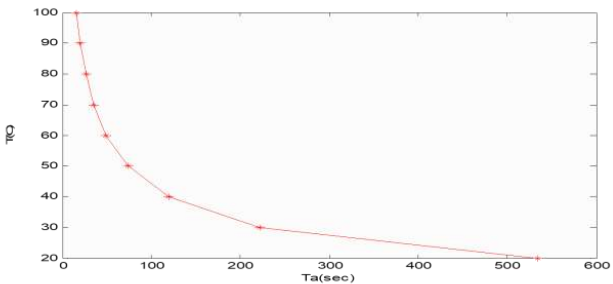
The fig.(3) relation between [Temperature( T ) and Time activation ( T_a )].
