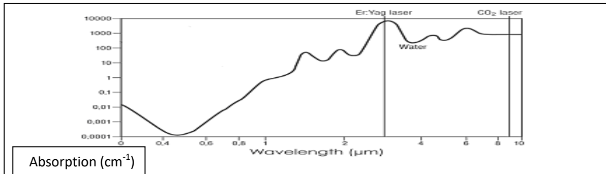
Fig(1) Absorption spectra of water .The absorption is highest at (3μm).
