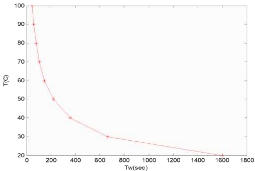
The fig. (2) relation between [Time whitening ( T_w ) and Tem.( ^{\circ}\text{C} )]
