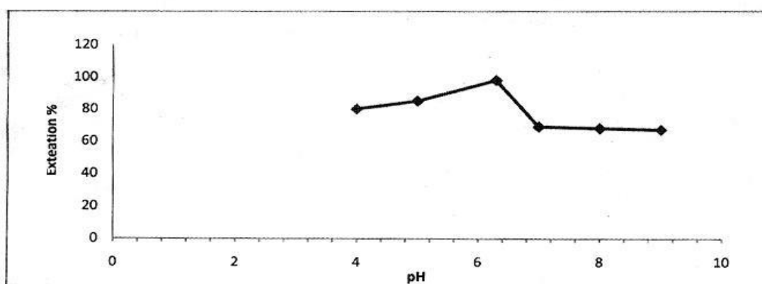
Fig ( 2) Extraction of Cu(II) as a Function of pH Choice of solvent
