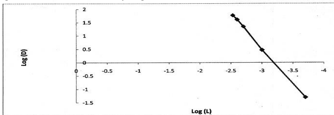
Fig( 6) Slope analysis method for Cu(II)DCH-18-Crown-6 Stability of complex
