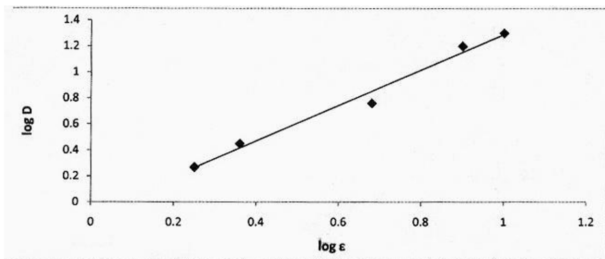
Fig (3) Effect of organic solvent on D distribution
