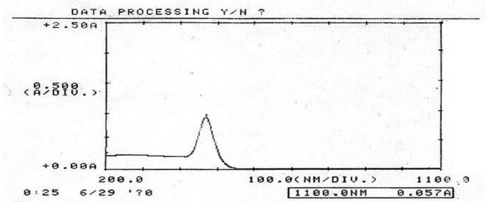
Fig(1) Absorption spectra Cu(II)DCH-18-crown-6 (Condition :Cu(II) 20 \mu g, Dicyclohexyl-18-crown-6 ( 10^{-3} M) ,PH(6.3)
