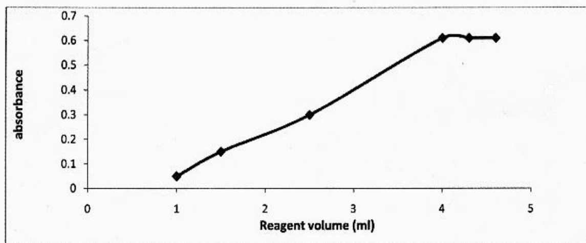
Fig (4) Effect reagent volume on the Extraction of Cu(II)
