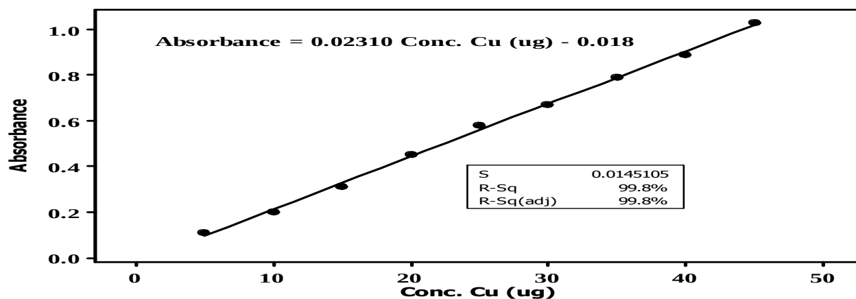
Fig (5) Calibration plot of Cu(II) DCH-18-Crown-6
