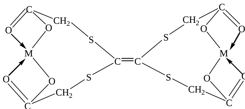
Dinuclear Complexes (1-4)
