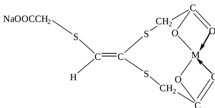
Mononuclear complexes(9-12)
