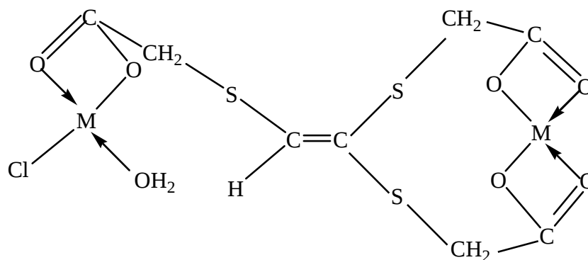
Dinuclear Complexes(5-8)
