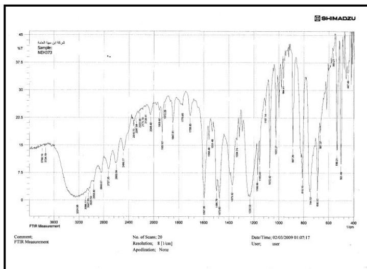
Fig. (4) FT-IR for compound (4)
