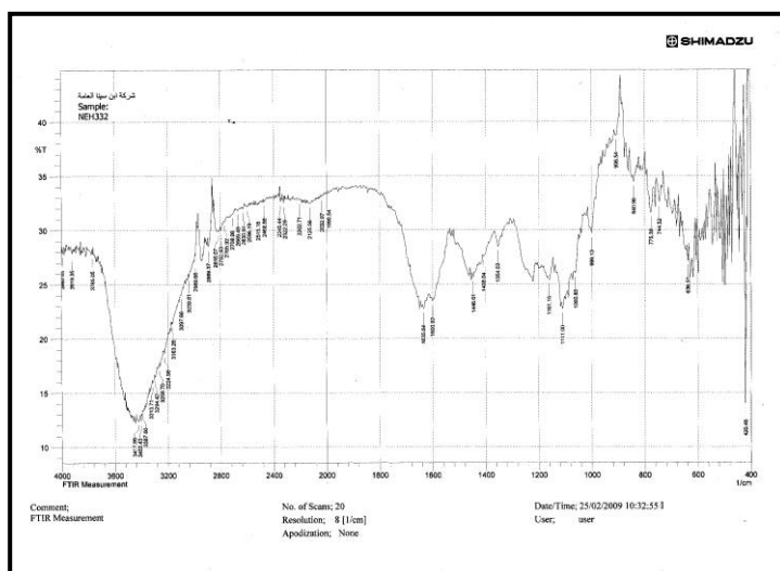
Fig. (6) FT-IR for compound (10)
