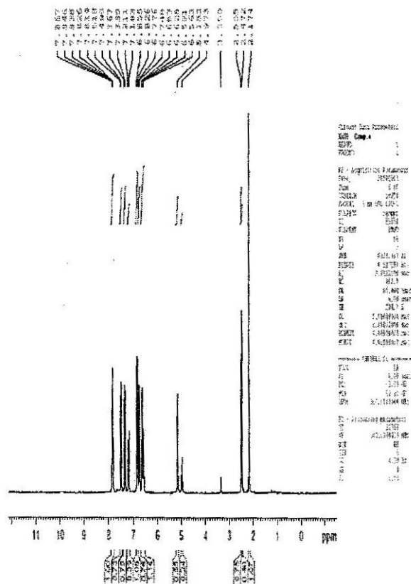
Fig. (8) HNMR Spectrum of Compound (4)
