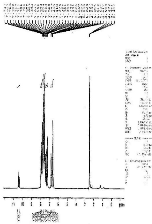
Fig. (10) HNMR Spectrum of Compound (10)
