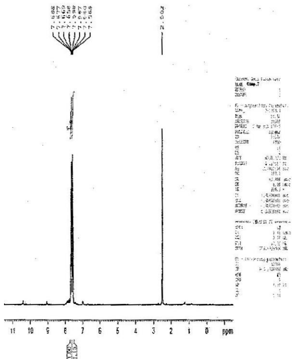
Fig. (9) HNMR Spectrum of Compound (7)
