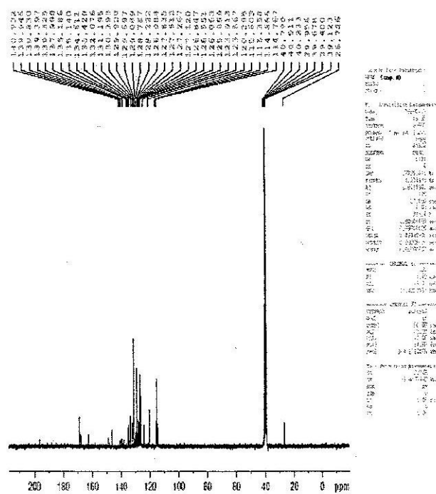
Fig. (14) 13 CNMR Spectrum of Compound (10)
