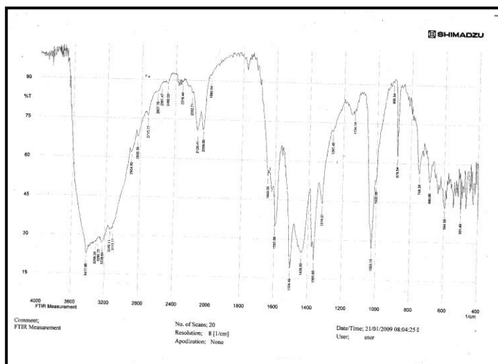
Fig. (2) FT-IR for compound (2)
