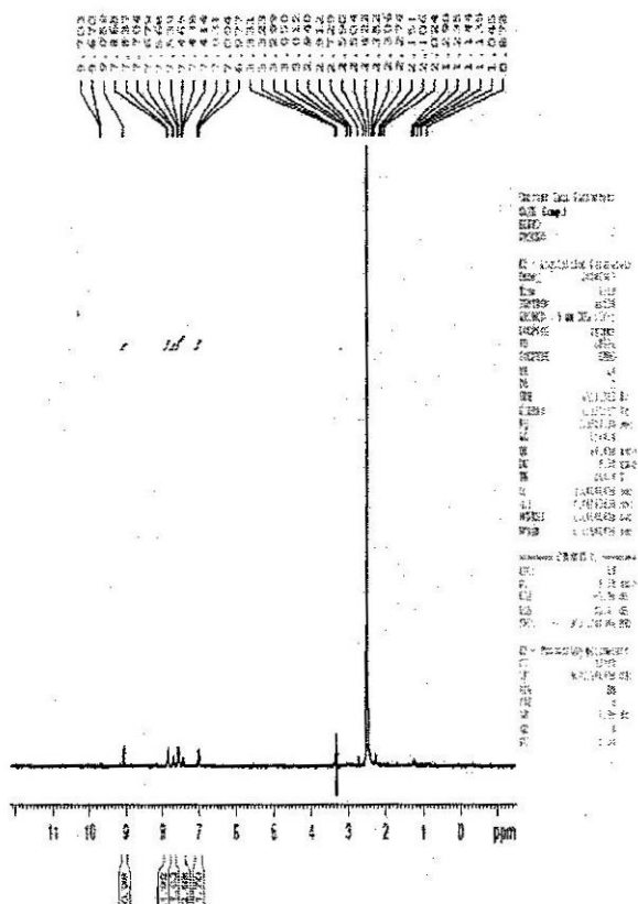
Fig. (7) HNMR Spectrum of Compound (1)
