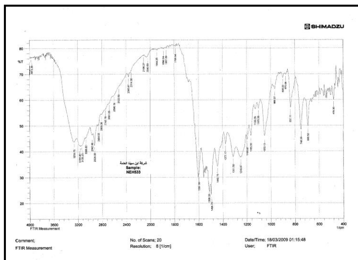
Fig. (1) FT-IR for compound (1)
