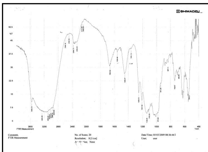
Fig. (5) FT-IR for compound (7)
