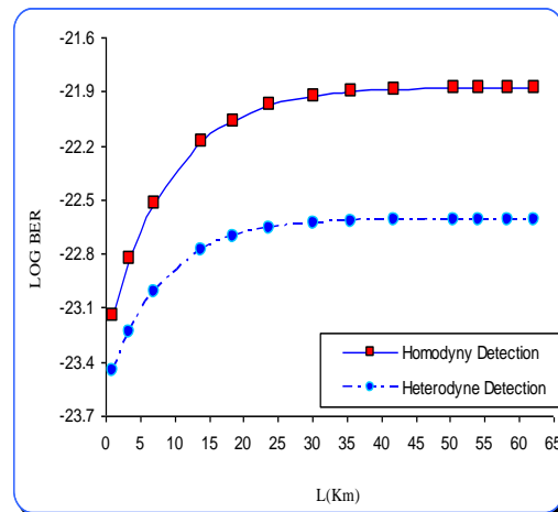
Figure 5: The variation of the logarithm of BER with the optical fiber length.
