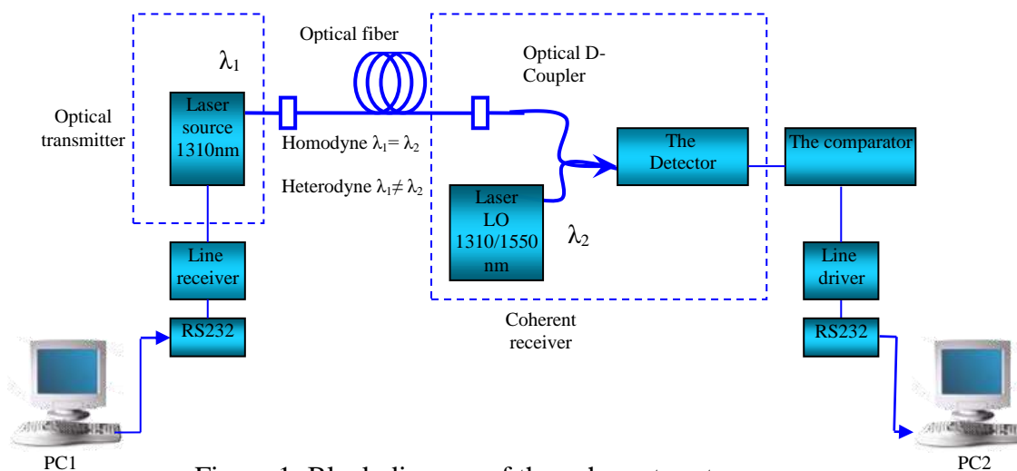
Figure 1: Block diagram of the coherent system
