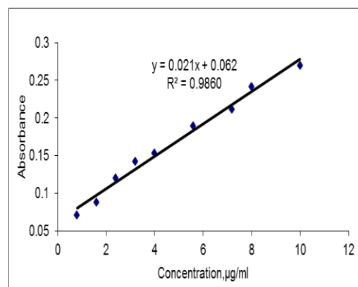
Fig. (3) Calibration graph for captopril.
