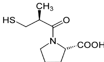
Fig. (1). Molecular structure of captopril.
