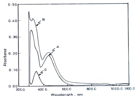
Fig.( 2). Absorption spectra of 300µg captopril / 25ml treated according to the recommended procedure and measured against (A) reagent blank, (B) distilled water and (C) reagent blank measured against distilled water.
