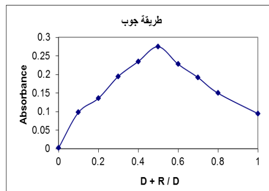
Fig (4.) : Job's method for captopril - dichlorone product
