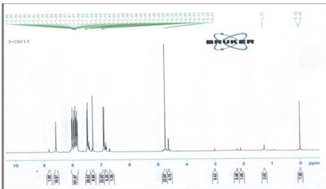
Fig (2): 1 H.N.M.R spectrum of compound [9].
