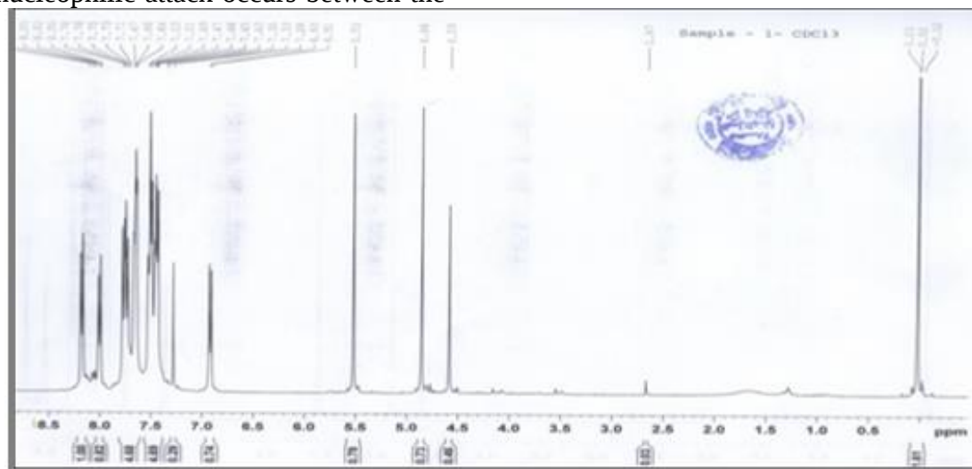
Fig (1): ^1\text{H-NMR} spectrum of compound [6].
