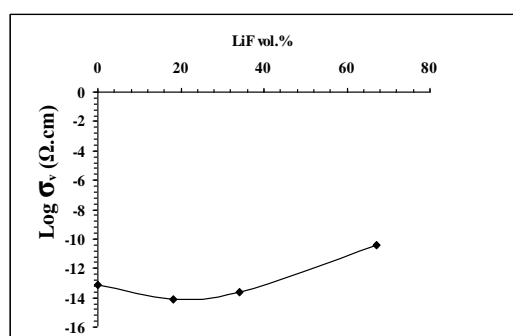
Fig. (4) variation of volume D.C electrical conductivity with LiF vol.% concentration.
