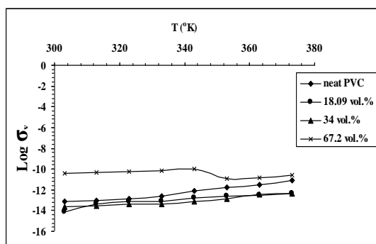
Fig. (7) variation of D.C electrical conductivity ( \sigma_v ) with temperature for (PVC-LiF) composite.
