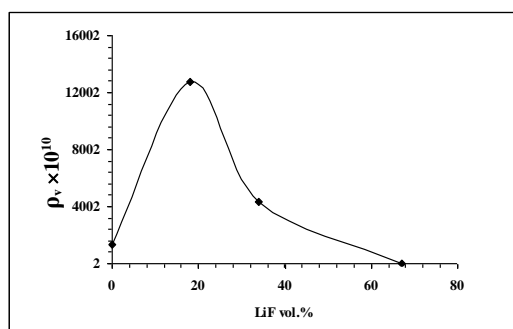
Fig. (3) variation of volume resistivity ( \rho_v ) with LiF vol.% concentration.
