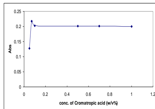
Fig. 6: The effect of the concentration of chromatropic acid reagent in (0.7M) of NaOH
