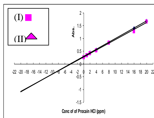
Fig. 11: the standard addition method For the batch method
