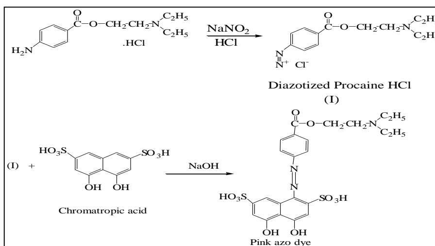
Scheme (1): reaction sequence
