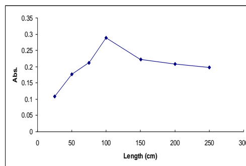
Fig. 10: The effect of the length of the reaction coil in (cm)
