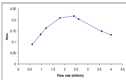
Fig. 8: The effect of the total flow rate (ml/min)
