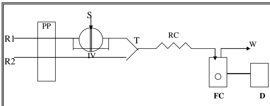
Fig. 4: A schematic diagram of FIA manifold
