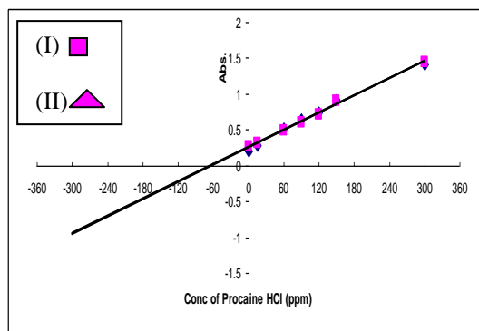
Fig. 12: the standard addition method for the FIA
