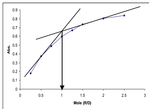
Fig. 2: Mole ratio plot of the reaction between diazotized Procaine HCl and chromatropic acid ( 1.38 \times 10^{-3} \text{M} )
