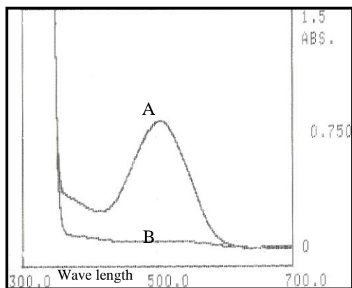
Fig. 1: Absorption spectra of the azo dye (20 ppm) against reagent blank (A) and blank against distilled water (B).
