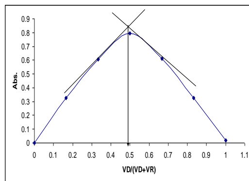
Fig. 3: Continuous variation plot of the reaction between diazotized Procaine HCl and chromatropic acid ( 1.38 \times 10^{-3} \text{M} )
