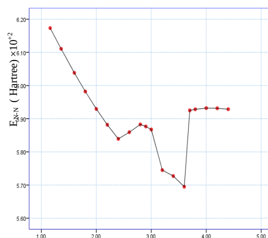
Fig (4): shows the E_{N-N} (Hartree) for C8b and C5a to acenaphthylene molecule .
