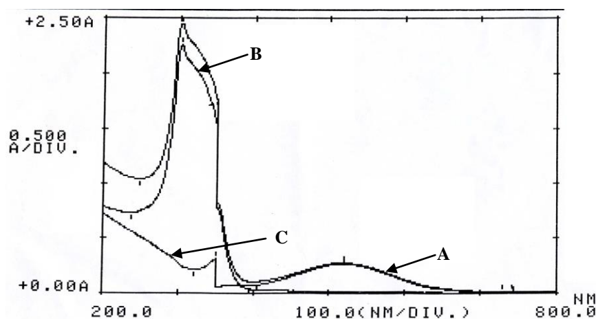
Fig. 2. Absorption spectra of 100 µg of p -aminophenol / 25 ml treated according to the recommended procedure and measured against (A) reagent blank, (B) distilled water and (C) reagent blank measured against distilled water.
