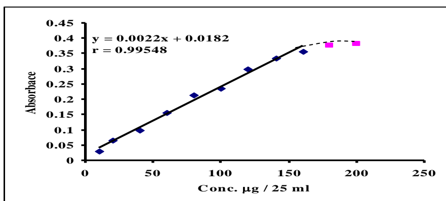
Fig. 1. Calibration graph of p -aminophenol determination
