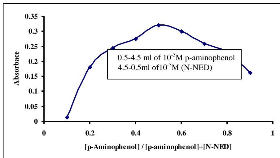
Fig. 3. Job's plot method of p -aminophenol-N-NED in the presence of \text{IO}_3^-
