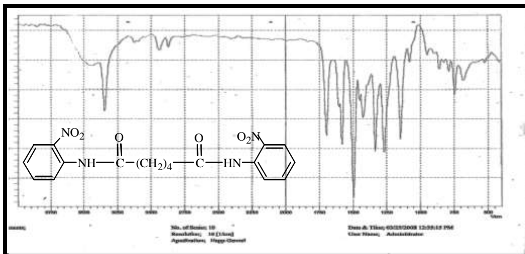
Fig. (4): FTIR spectrum of compound (4)
