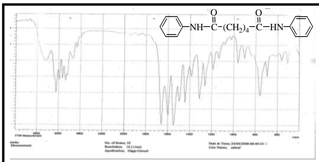
Fig. (3): FTIR spectrum of compound (3)
