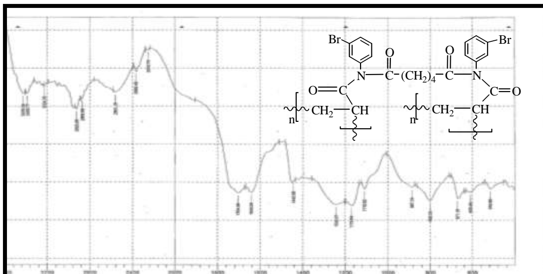
Fig. (7): FTIR spectrum of resin (7)
