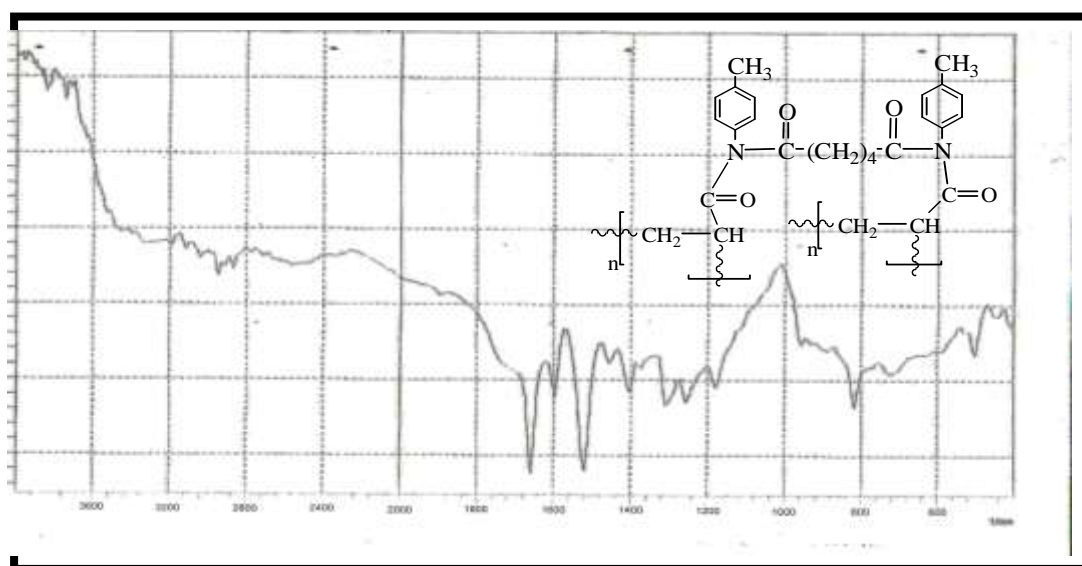
Fig. (6): FTIR spectrum of resin (6)
