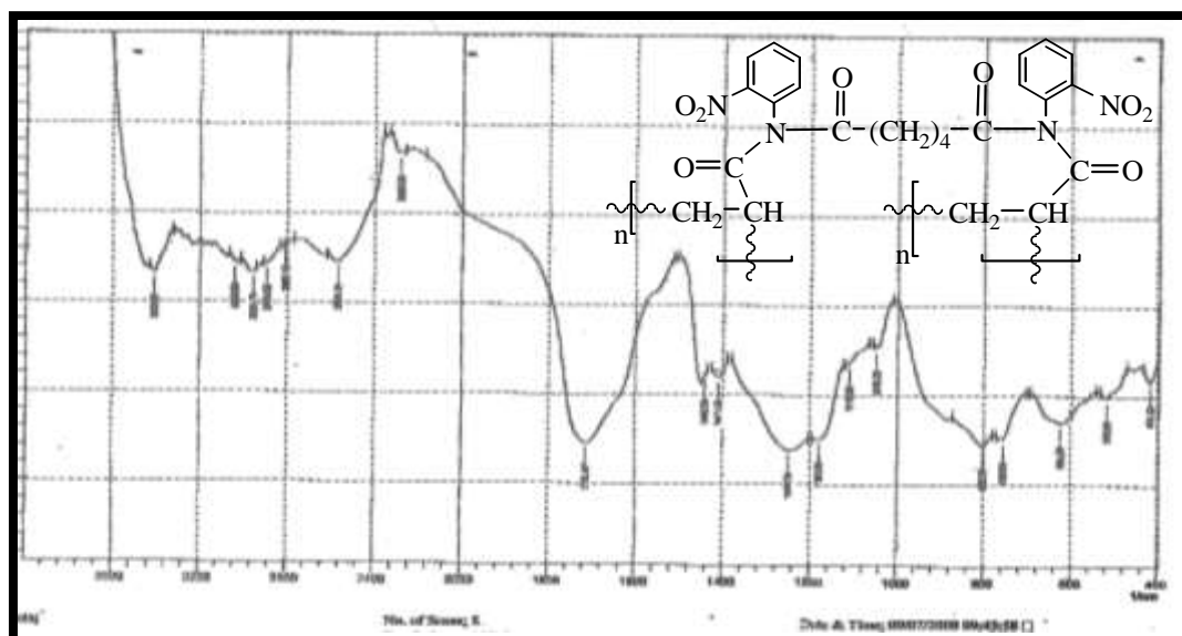
Fig. (9): FTIR spectrum of resin (9)
