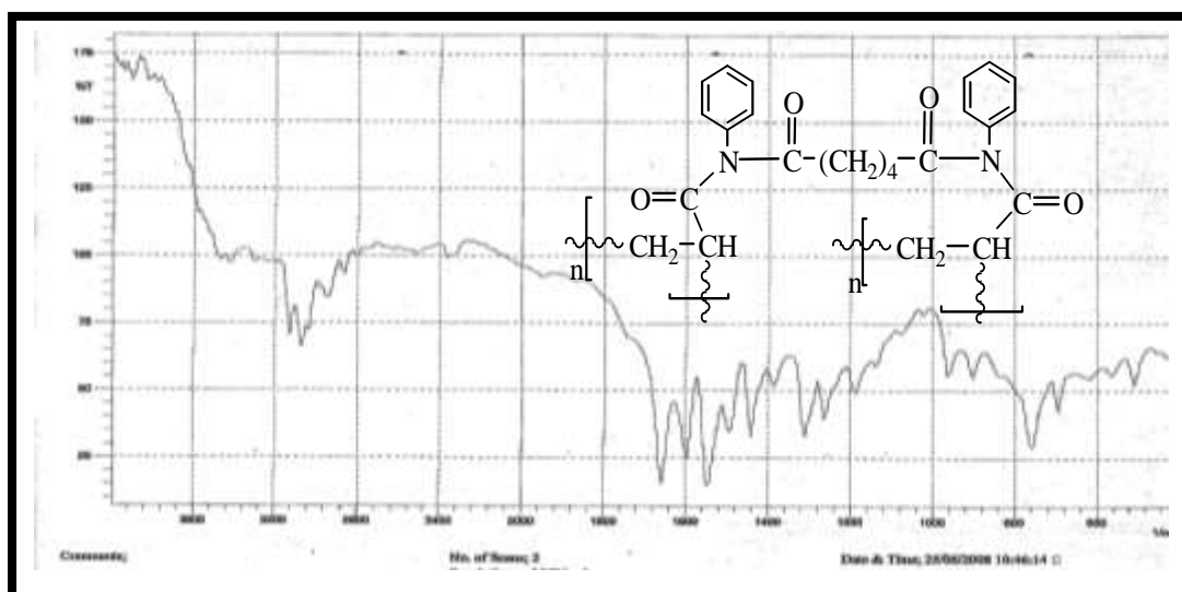
Fig. (8): FTIR spectrum of resin (8)
