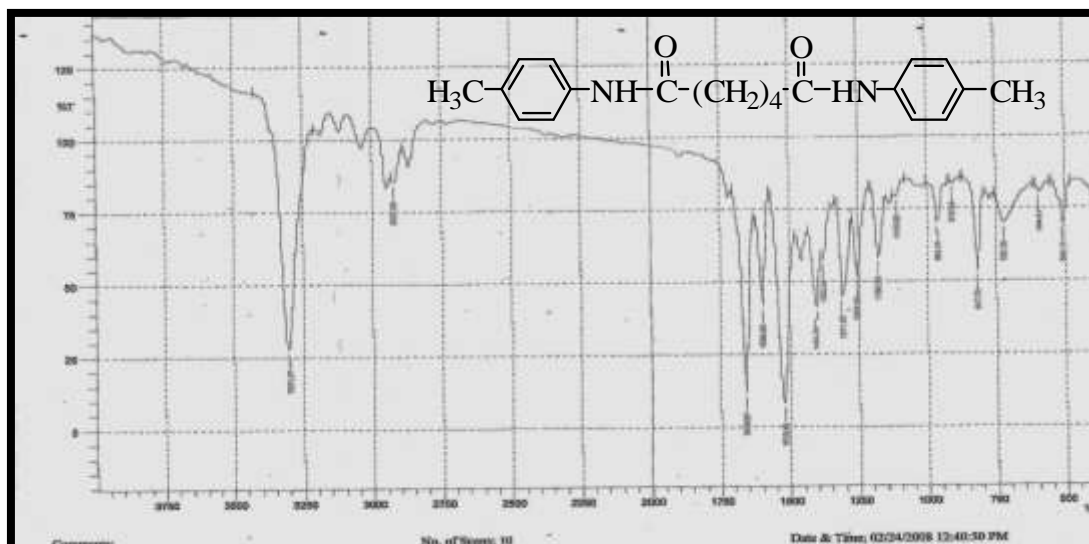
Fig. (1): FTIR spectrum of compound (1)
