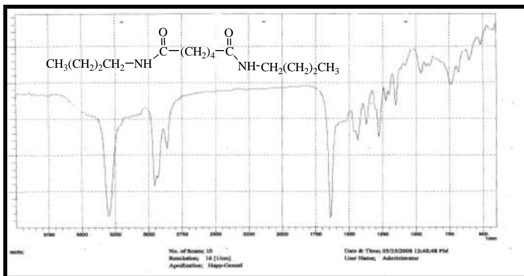
Fig.(5):FTIR spectrum of compound (5)
