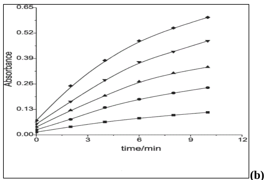
Figure (3): (a) Absorption spectrum of CdO nanoparticles–propyl mercaptan during 0–1200 (s). (b) Absorption curve against time for CdO nanoparticles–propyl mercaptan at maximum wavelength.
