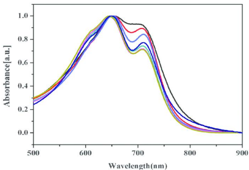
Figure (2): (a) Absorption spectrum of CdO nanoparticles–benzyl mercaptan during 0–1200 (s). (b) Absorption curve against time for CdO nanoparticles–benzyl mercaptan at maximum wavelength.
