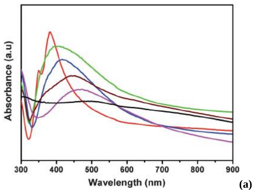
Figure (1): (a) Absorption spectrum of CdO nanoparticles–phenyl mercaptan during 0–1200 (s). (b) Absorption curve against time for CdO nanoparticles–phenyl mercaptan at maximum wavelength.
