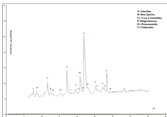
Fig. 8: X-Ray Diagram of ceramic disc filter.
