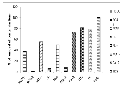
Fig. 12. % of removal of different contaminations by CP.
