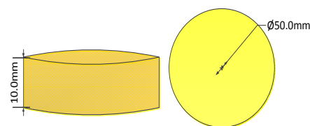
Fig.1– Filter Ceramic Disc Dimensions
