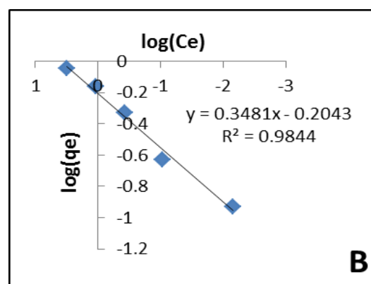
Figs.11.A: Langmuir graph, Freundlich graph of data for adsorption capacity of Co.
