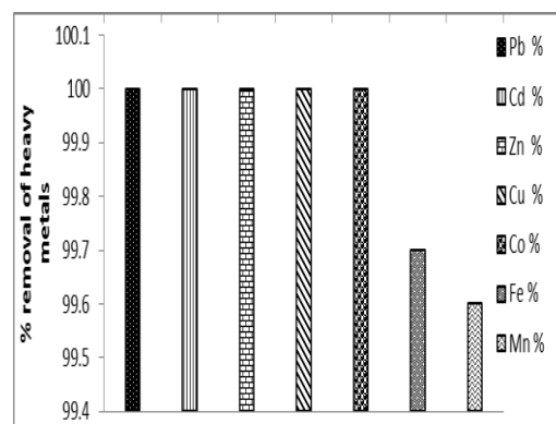
Fig 9: % of removal of heavy metals at concentration 1\text{mg/l} .
