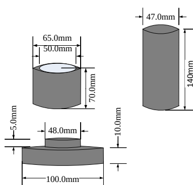
Fig.2. Manufactured Carbonate Steel Mold.
