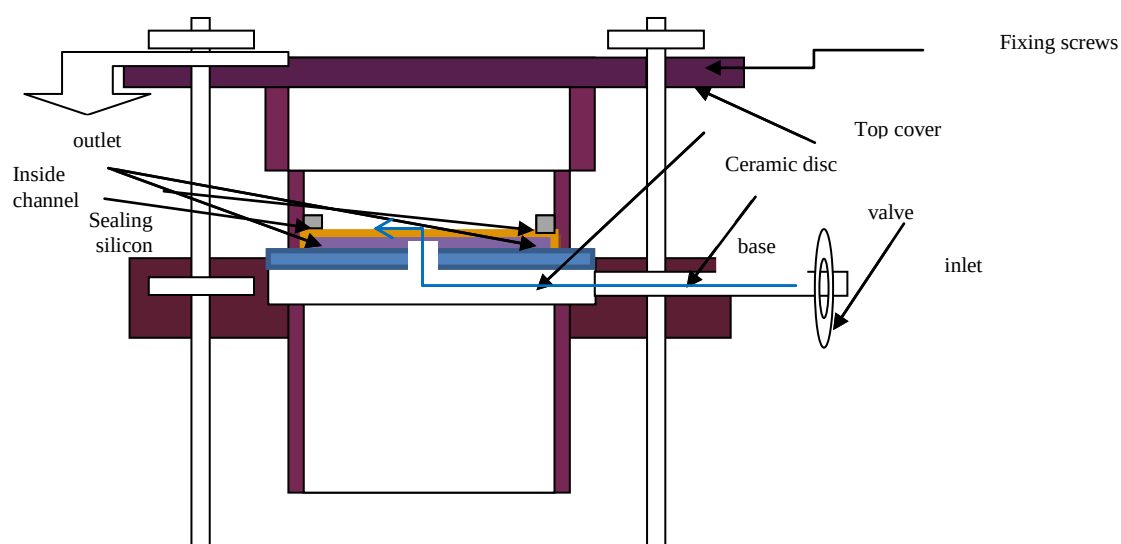
Fig. 5. Schematic diagram of hydraulic conductivity test equipment.
