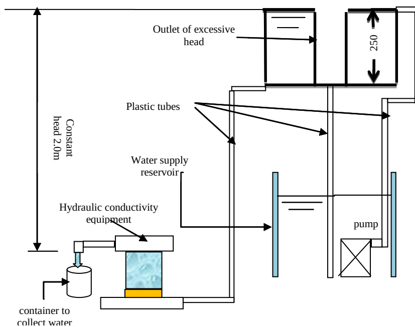
Fig.7. Schematic diagram of hydraulic conductivity test rig.
