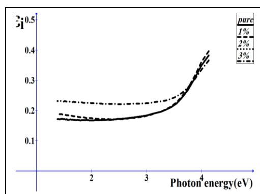
Fig. (7) Imaginary part versus photo energy for the as deposited films.
