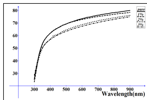
Fig. (1) Transmittance versus wavelength for the as deposited films.
