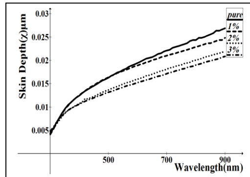
Fig. (5) Skin depth versus wavelength for the as deposited films.
