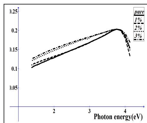
Fig. (2) Reflectance versus photo energy for the as deposited films.
