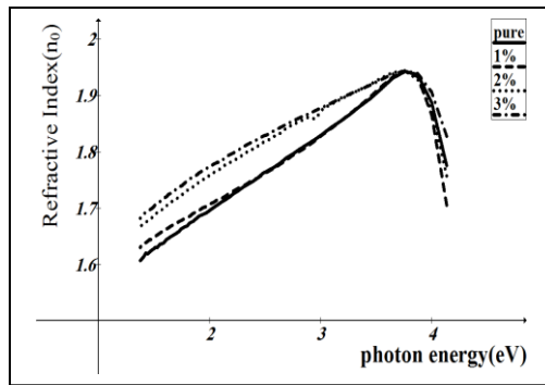
Fig. (3) Refractive index versus photo energy for the as deposited films.
