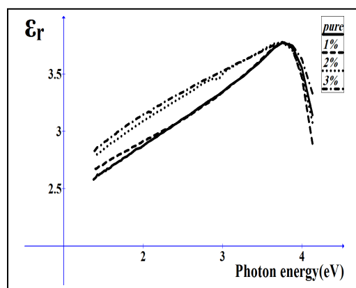
Fig. (6) Real part versus photo energy for the as deposited films.
