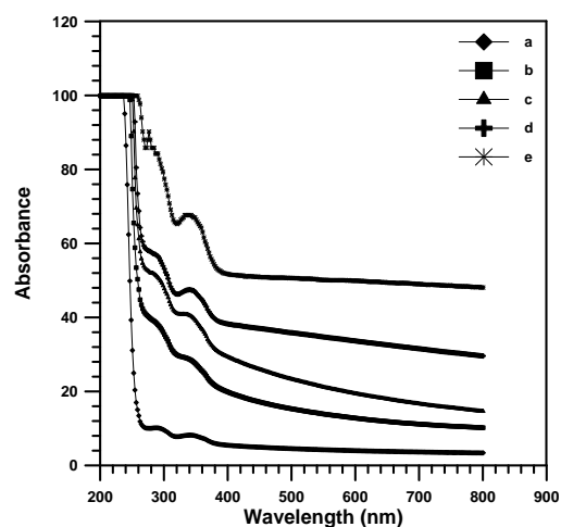
Fig.(1) Absorption spectra of (a-e) PMMA sample.
