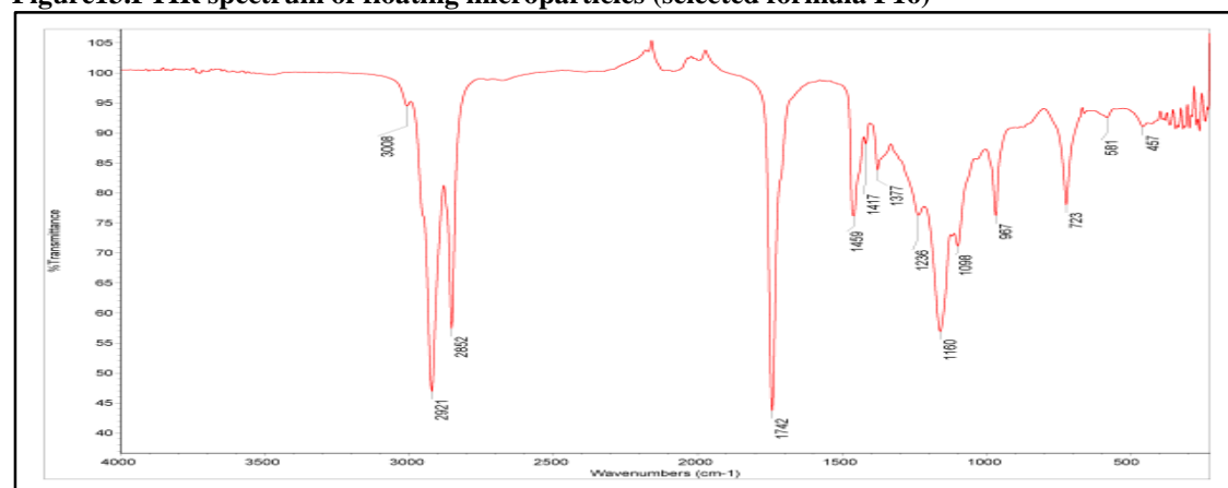
Figure 14. FTIR spectrum of safflower oil. (27)
