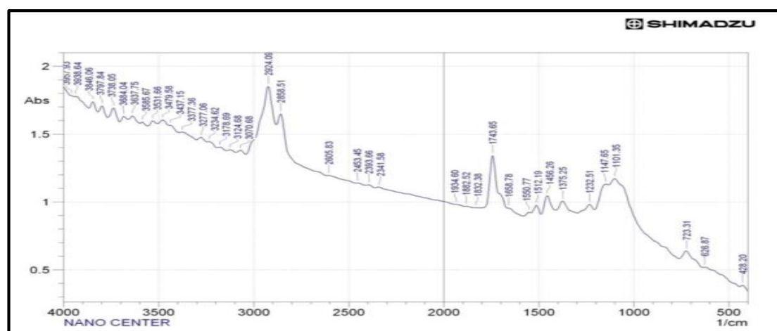
Figure13.FTIR spectrum of floating microparticles (selected formula F16)
