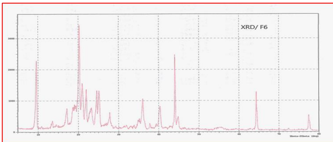
Figure 15. XRD of pure ITZ.
