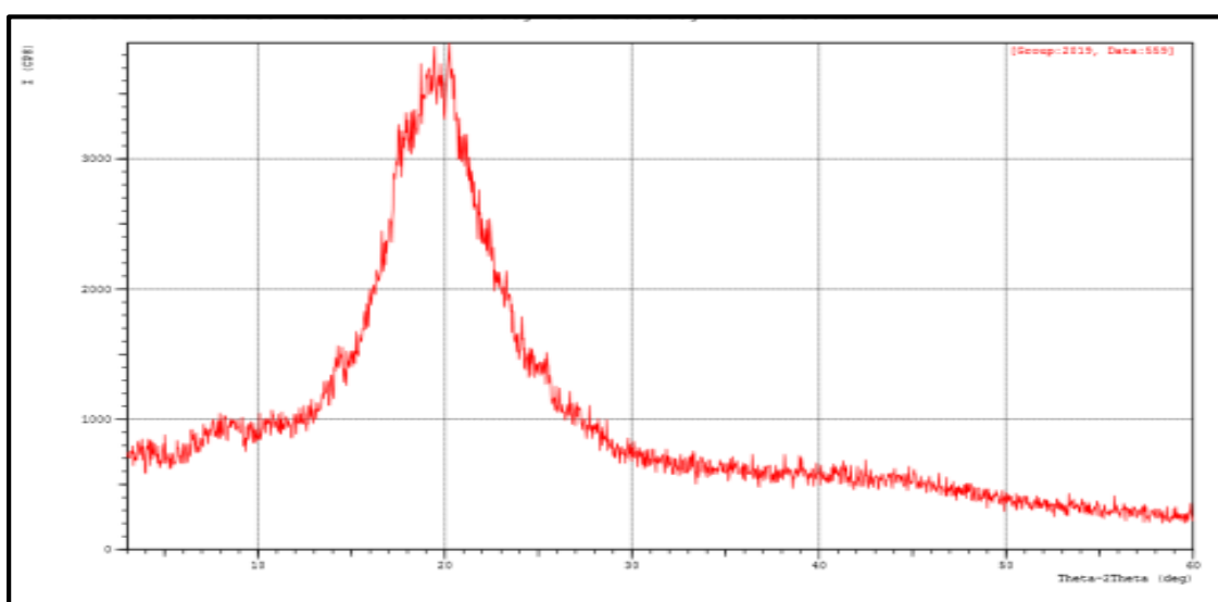
Figure 16.XRD of ITZ selected formula (F16)
