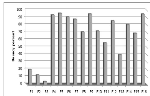
Figure 6. Bouncy percent of ITZ floating microparticles
