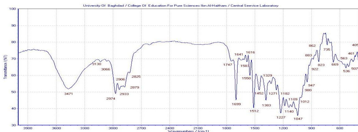
Figure 12. FTIR spectrum of the physical mixture of drug, EC and HPMC 15cps.
